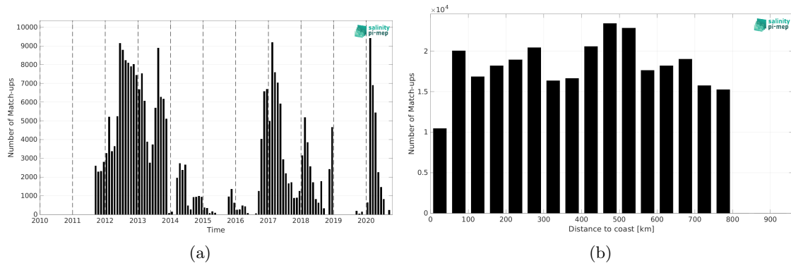
Figure 2: Number of match-ups between Surface drifters and SMAP SSS L4 OI v3 - Monthly (ESR) SSS as a function of time (a) and as function of the distance to coast (b) over the SMOS coastal zone (<800km) 60N-60S Pi-MEP region and for the full satellite product period.
