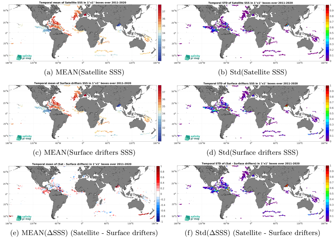
Figure 6: Temporal mean (left) and Std (right) of SSS from SMAP SSS L4 OI v3 - Monthly (ESR) (top), Surface drifters (middle), and of \Delta SSS (Satellite - Surface drifters). Only match-up pairs are used to generate these maps.
