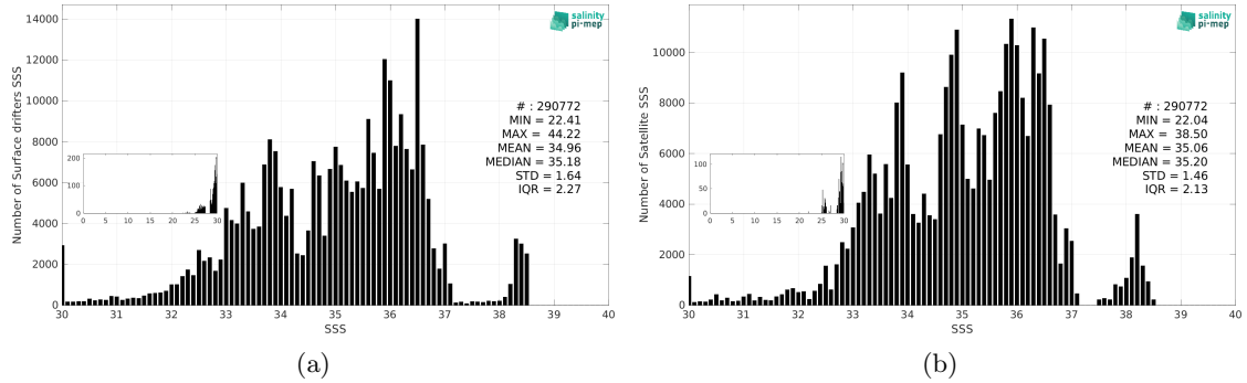
Figure 3: Histograms of SSS from Surface drifters (a) and SMAP SSS L4 OI v3 - Monthly (ESR) (b) considering all match-up pairs per bins of 0.1 over the SMOS coastal zone (<800km) 60N-60S Pi-MEP region and for the full satellite product period.
