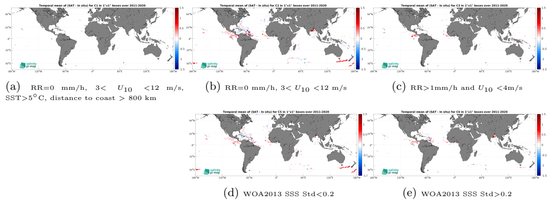
Figure 13: Temporal mean gridded over spatial boxes of size 1^\circ \times 1^\circ of \Delta SSS (SMAP SSS L4 OI v3 - Monthly (ESR) - Surface drifters) for 5 different subdatasets corresponding to:RR=0 mm/h, 3 < U_{10} < 12 m/s, SST >5^\circ\text{C} , distance to coast > 800 km (a), RR=0 mm/h, 3 < U_{10} < 12 m/s (b), RR >1 mm/h and U_{10} < 4 m/s (c), WOA2013 SSS Std <0.2 (d), WOA2013 SSS Std >0.2 (e).
