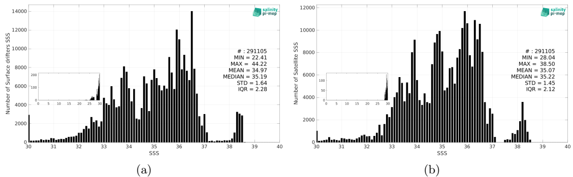
Figure 3: Histograms of SSS from Surface drifters (a) and SMAP SSS L4 OI v3 - Monthly (ESR) (b) considering all match-up pairs per bins of 0.1 over the SMOS coastal zone (<800km) 60N-60S Pi-MEP region and for the full satellite product period.
