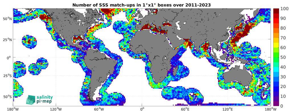
Figure 5: Number of SSS match-ups between Argo SSS and the SMAP SSS L4 OI v3 - Monthly (ESR) SSS product for the SMOS coastal zone (<800km) 60N-60S Pi-MEP region over 1^\circ \times 1^\circ boxes and for the full satellite product period.
