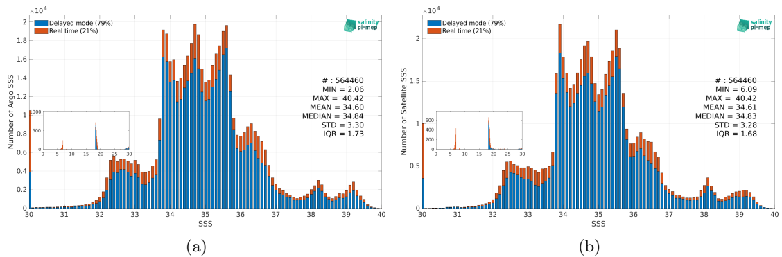
Figure 3: Histograms of SSS from Argo (a) and SMAP SSS L4 OI v3 - Monthly (ESR) (b) considering all match-up pairs per bins of 0.1 over the SMOS coastal zone (<800km) 60N-60S Pi-MEP region and for the full satellite product period.
