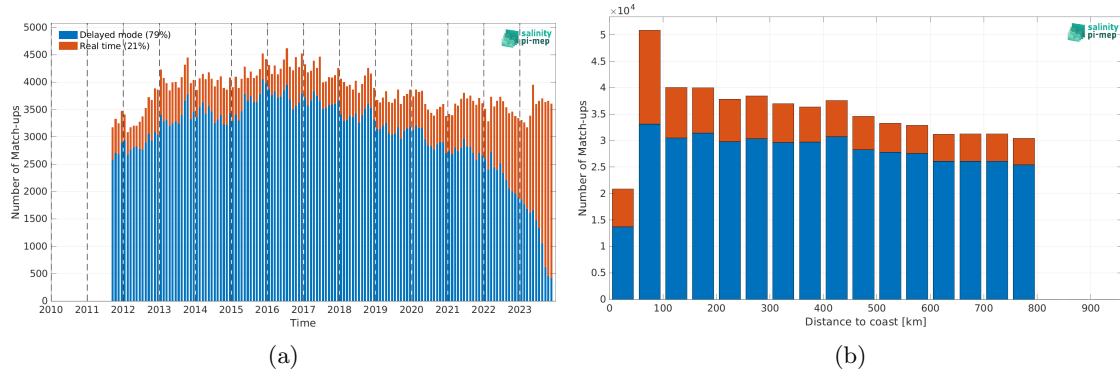
Figure 2: Number of match-ups between Argo and SMAP SSS L4 OI v3 - Monthly (ESR) SSS as a function of time (a) and as function of the distance to coast (b) over the SMOS coastal zone (<800km) 60N-60S Pi-MEP region and for the full satellite product period.
