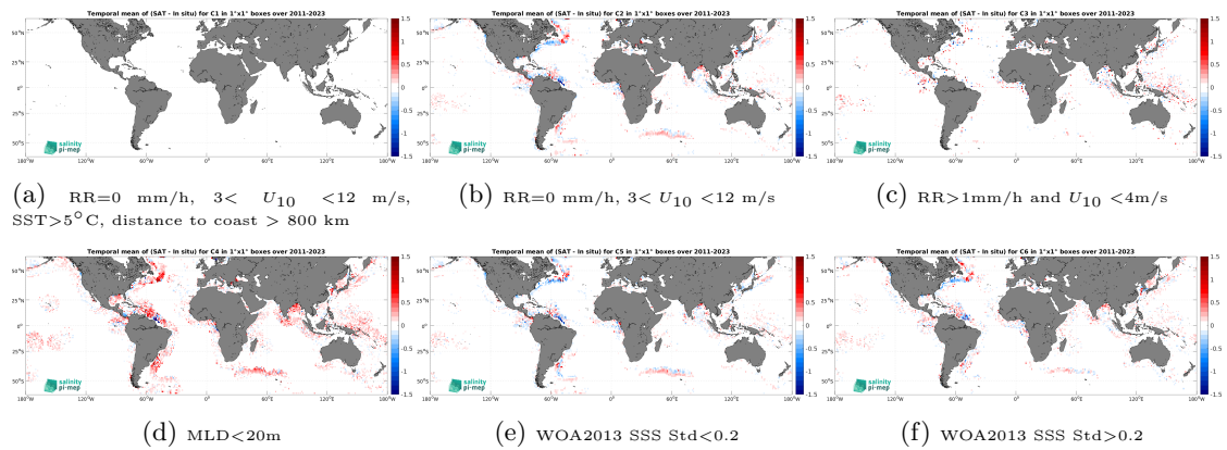
Figure 14: Temporal mean gridded over spatial boxes of size 1^\circ \times 1^\circ of \Delta SSS (SMAP SSS L4 OI v3 - Monthly (ESR) - Argo) for 6 different subdatasets corresponding to:RR=0 mm/h, 3 < U_{10} < 12 m/s, SST > 5^\circ\text{C} , distance to coast > 800 km (a), RR=0 mm/h, 3 < U_{10} < 12 m/s (b), RR > 1 mm/h and U_{10} < 4 m/s (c),MLD < 20 m (d),WOA2013 SSS Std < 0.2 (e),WOA2013 SSS Std > 0.2 (f).
