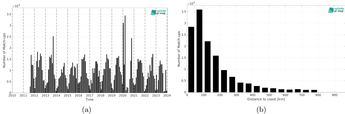
Figure 2: Number of match-ups between TSG (SAMOS) and SMAP SSS L4 OI v3 - Daily (ESR) SSS as a function of time (a) and as function of the distance to coast (b) over the SMOS coastal zone (<800km) 60N-60S Pi-MEP region and for the full satellite product period.
