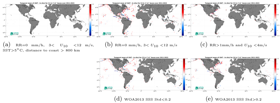
Figure 14: Temporal mean gridded over spatial boxes of size 1^\circ \times 1^\circ of \Delta\text{SSS} (SMAP SSS L4 OI v3 - Daily (ESR) - TSG (SAMOS)) for 5 different subdatasets corresponding to:RR=0 mm/h, 3 < U_{10} < 12 m/s, SST>5°C, distance to coast > 800 km (a), RR=0 mm/h, 3 < U_{10} < 12 m/s (b), RR>1mm/h and U_{10} < 4 m/s (c), WOA2013 SSS Std<0.2 (d), WOA2013 SSS Std>0.2 (e).
