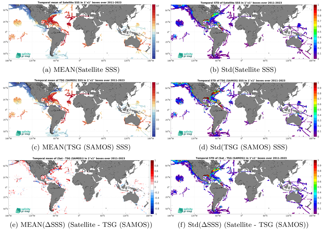
Figure 7: Temporal mean (left) and Std (right) of SSS from SMAP SSS L4 OI v3 - Daily (ESR) (top), TSG (SAMOS) (middle), and of \Delta SSS (Satellite - TSG (SAMOS)). Only match-up pairs are used to generate these maps.
