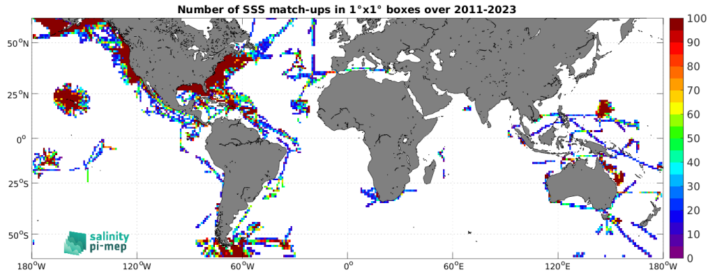
Figure 5: Number of SSS match-ups between TSG (SAMOS) SSS and the SMAP SSS L4 OI v3 - Daily (ESR) SSS product for the SMOS coastal zone (<800km) 60N-60S Pi-MEP region over 1^\circ \times 1^\circ boxes and for the full satellite product period.
