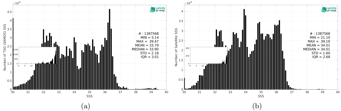
Figure 3: Histograms of SSS from TSG (SAMOS) (a) and SMAP SSS L4 OI v3 - Daily (ESR) (b) considering all match-up pairs per bins of 0.1 over the SMOS coastal zone (<800km) 60N-60S Pi-MEP region and for the full satellite product period.
