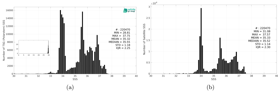
Figure 3: Histograms of SSS from TSG (Polarstern) (a) and SMAP SSS L4 OI v3 - Daily (ESR) (b) considering all match-up pairs per bins of 0.1 over the SMOS coastal zone (<800km) 60N-60S Pi-MEP region and for the full satellite product period.
