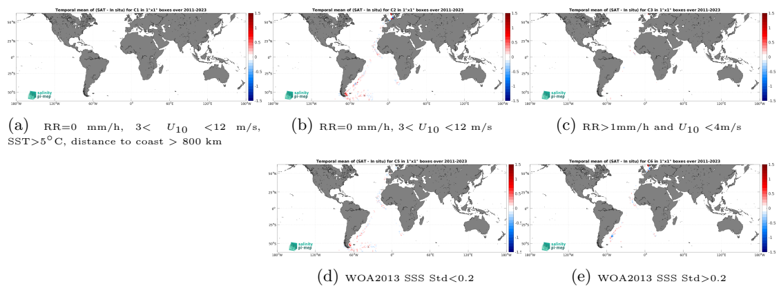
Figure 14: Temporal mean gridded over spatial boxes of size 1^\circ \times 1^\circ of \Delta\text{SSS} (SMAP SSS L4 OI v3 - Daily (ESR) - TSG (Polarstern)) for 5 different subdatasets corresponding to:RR=0 mm/h, 3 < U_{10} < 12 m/s, SST>5°C, distance to coast > 800 km (a), RR=0 mm/h, 3 < U_{10} < 12 m/s (b), RR>1mm/h and U_{10} < 4 m/s (c), WOA2013 SSS Std<0.2 (d), WOA2013 SSS Std>0.2 (e).
