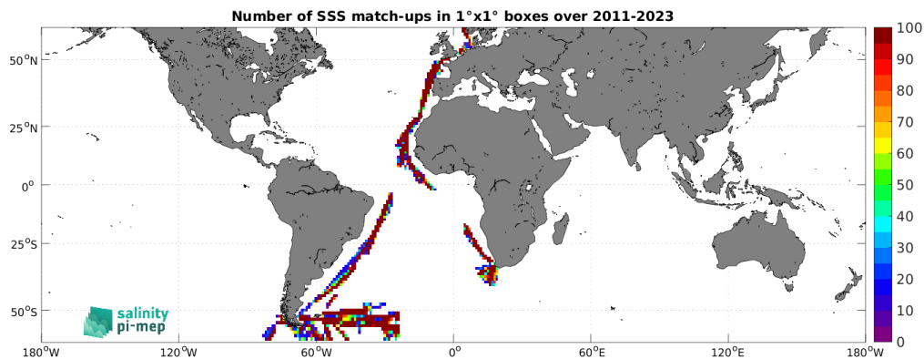
Figure 5: Number of SSS match-ups between TSG (Polarstern) SSS and the SMAP SSS L4 OI v3 - Daily (ESR) SSS product for the SMOS coastal zone (<800km) 60N-60S Pi-MEP region over 1^\circ \times 1^\circ boxes and for the full satellite product period.
