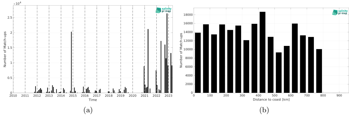
Figure 2: Number of match-ups between TSG (Polarstern) and SMAP SSS L4 OI v3 - Daily (ESR) SSS as a function of time (a) and as function of the distance to coast (b) over the SMOS coastal zone (<800km) 60N-60S Pi-MEP region and for the full satellite product period.
