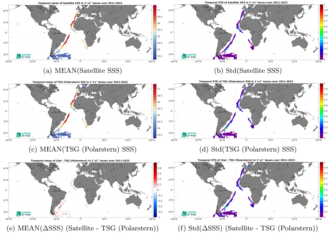
Figure 7: Temporal mean (left) and Std (right) of SSS from SMAP SSS L4 OI v3 - Daily (ESR) (top), TSG (Polarstern) (middle), and of \Delta SSS (Satellite - TSG (Polarstern)). Only match-up pairs are used to generate these maps.
