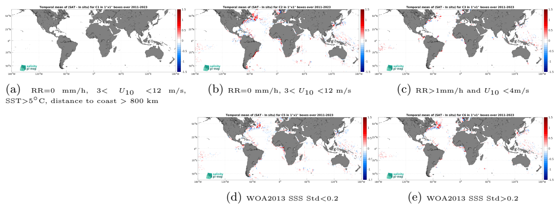
Figure 14: Temporal mean gridded over spatial boxes of size 1^\circ \times 1^\circ of \Delta\text{SSS} (SMAP SSS L4 OI v3 - Daily (ESR) - TSG (LEGOS-DM)) for 5 different subdatasets corresponding to:RR=0 mm/h, 3 < U_{10} < 12 m/s, SST >5^\circ\text{C} , distance to coast > 800 km (a), RR=0 mm/h, 3 < U_{10} < 12 m/s (b), RR >1 mm/h and U_{10} < 4 m/s (c), WOA2013 SSS Std <0.2 (d), WOA2013 SSS Std >0.2 (e).
