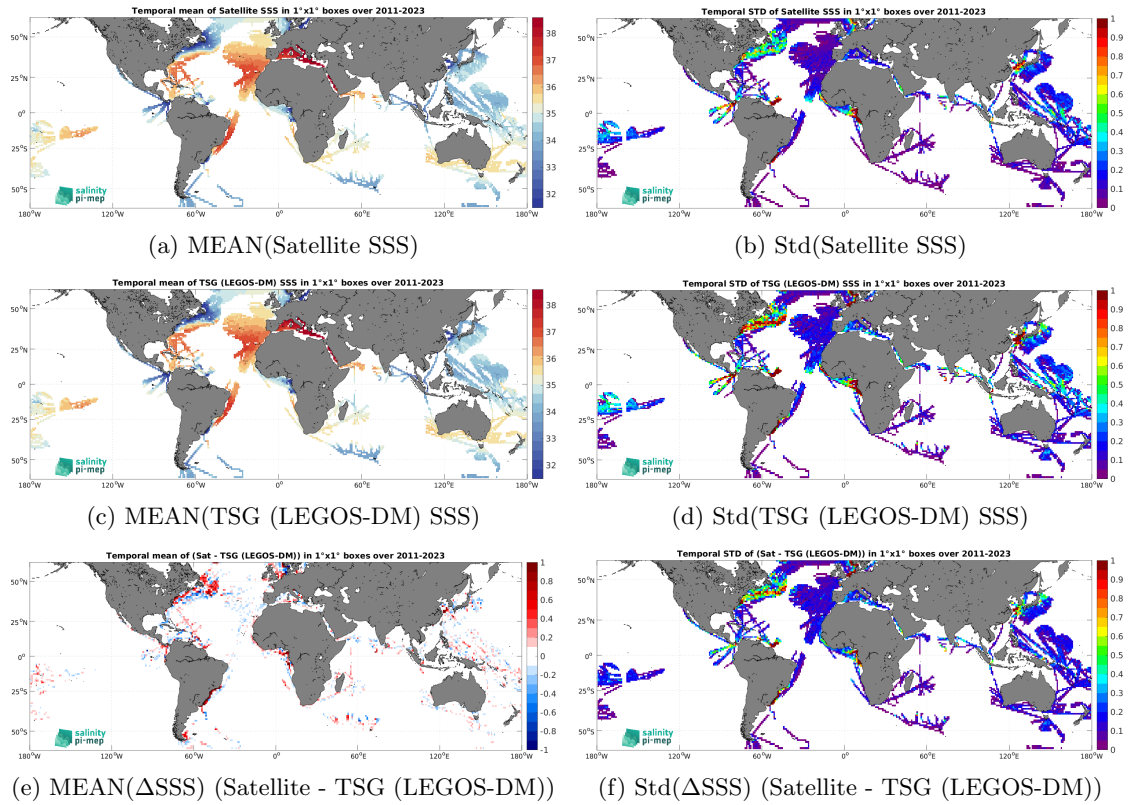
Figure 7: Temporal mean (left) and Std (right) of SSS from SMAP SSS L4 OI v3 - Daily (ESR) (top), TSG (LEGOS-DM) (middle), and of \Delta SSS (Satellite - TSG (LEGOS-DM)). Only match-up pairs are used to generate these maps.
