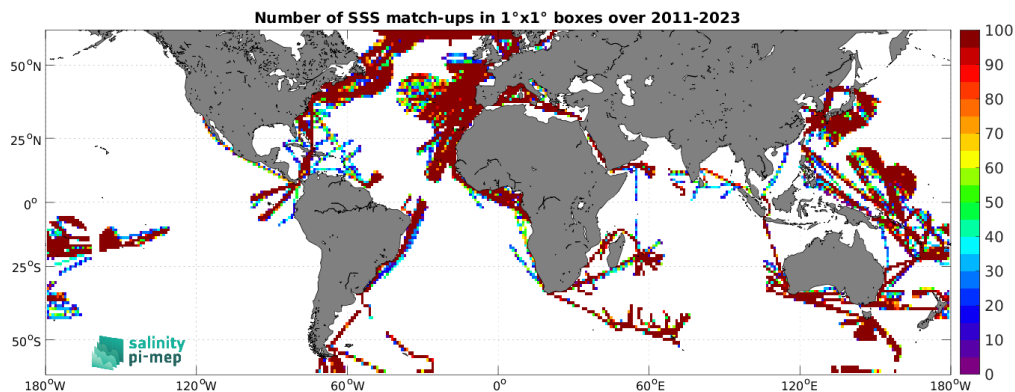
Figure 5: Number of SSS match-ups between TSG (LEGOS-DM) SSS and the SMAP SSS L4 OI v3 - Daily (ESR) SSS product for the SMOS coastal zone (<800km) 60N-60S Pi-MEP region over 1^\circ \times 1^\circ boxes and for the full satellite product period.
