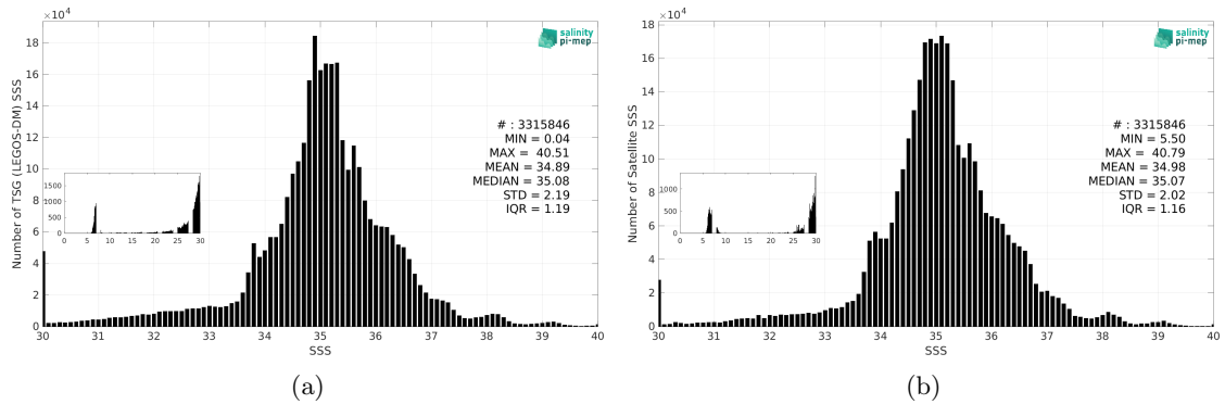
Figure 3: Histograms of SSS from TSG (LEGOS-DM) (a) and SMAP SSS L4 OI v3 - Daily (ESR) (b) considering all match-up pairs per bins of 0.1 over the SMOS coastal zone (<800km) 60N-60S Pi-MEP region and for the full satellite product period.
