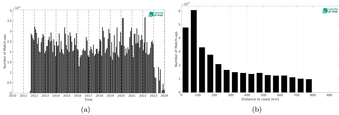
Figure 2: Number of match-ups between TSG (LEGOS-DM) and SMAP SSS L4 OI v3 - Daily (ESR) SSS as a function of time (a) and as function of the distance to coast (b) over the SMOS coastal zone (<800km) 60N-60S Pi-MEP region and for the full satellite product period.
