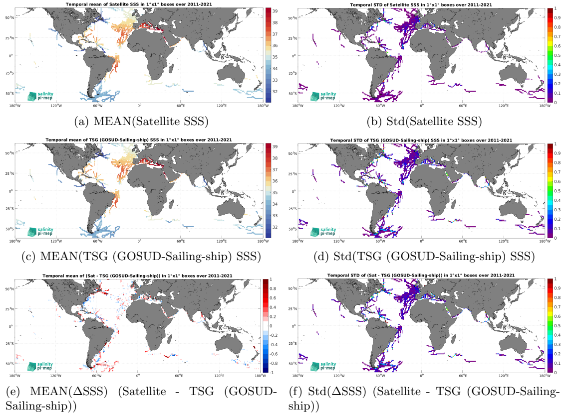
Figure 7: Temporal mean (left) and Std (right) of SSS from SMAP SSS L4 OI v3 - Daily (ESR) (top), TSG (GOSUD-Sailing-ship) (middle), and of \Delta SSS (Satellite - TSG (GOSUD-Sailing-ship)). Only match-up pairs are used to generate these maps.
