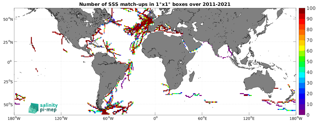
Figure 5: Number of SSS match-ups between TSG (GOSUD-Sailing-ship) SSS and the SMAP SSS L4 OI v3 - Daily (ESR) SSS product for the SMOS coastal zone (<800km) 60N-60S Pi-MEP region over 1^{\circ} \times 1^{\circ} boxes and for the full satellite product period.
