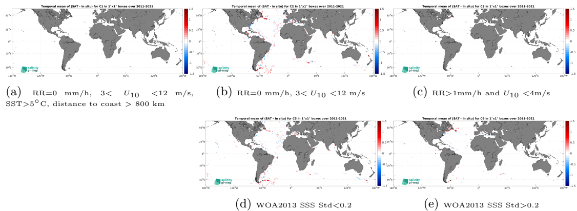
Figure 14: Temporal mean gridded over spatial boxes of size 1^\circ \times 1^\circ of \Delta\text{SSS} (SMAP SSS L4 OI v3 - Daily (ESR) - TSG (GOSUD-Sailing-ship)) for 5 different subdatasets corresponding to:RR=0 mm/h, 3 < U_{10} < 12 m/s, SST >5^\circ\text{C} , distance to coast > 800 km (a), RR=0 mm/h, 3 < U_{10} < 12 m/s (b), RR >1 mm/h and U_{10} < 4 m/s (c), WOA2013 SSS Std <0.2 (d), WOA2013 SSS Std >0.2 (e).
