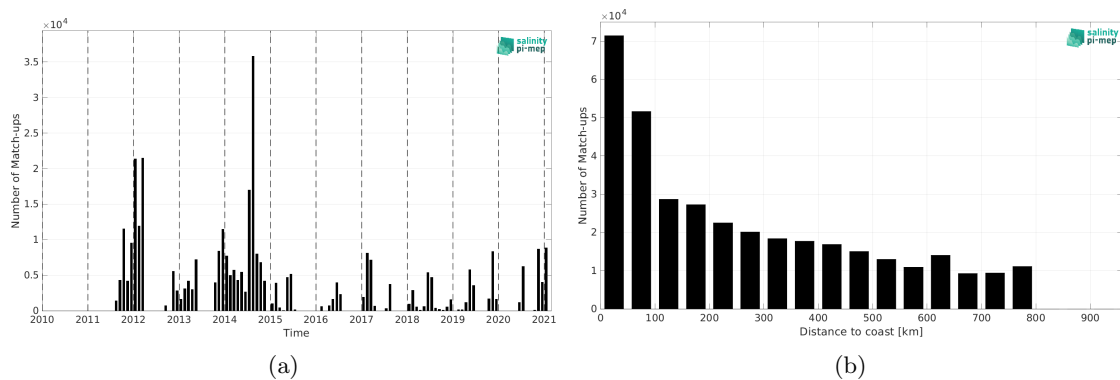
Figure 2: Number of match-ups between TSG (GOSUD-Sailing-ship) and SMAP SSS L4 OI v3 - Daily (ESR) SSS as a function of time (a) and as function of the distance to coast (b) over the SMOS coastal zone (<800km) 60N-60S Pi-MEP region and for the full satellite product period.
