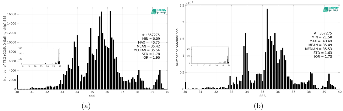
Figure 3: Histograms of SSS from TSG (GOSUD-Sailing-ship) (a) and SMAP SSS L4 OI v3 - Daily (ESR) (b) considering all match-up pairs per bins of 0.1 over the SMOS coastal zone (<800km) 60N-60S Pi-MEP region and for the full satellite product period.
