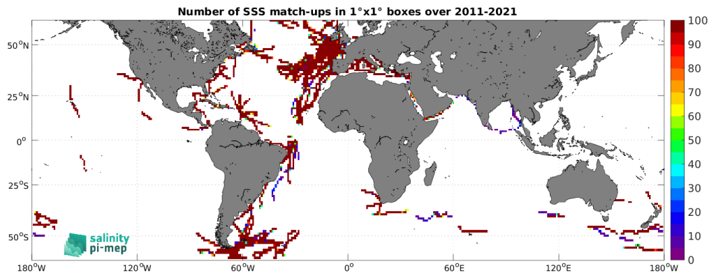
Figure 5: Number of SSS match-ups between TSG (GOSUD-Sailing-ship) SSS and the SMAP SSS L4 OI v3 - Daily (ESR) SSS product for the SMOS coastal zone ( <800\text{km} ) 60N-60S Pi-MEP region over 1^\circ \times 1^\circ boxes and for the full satellite product period.
