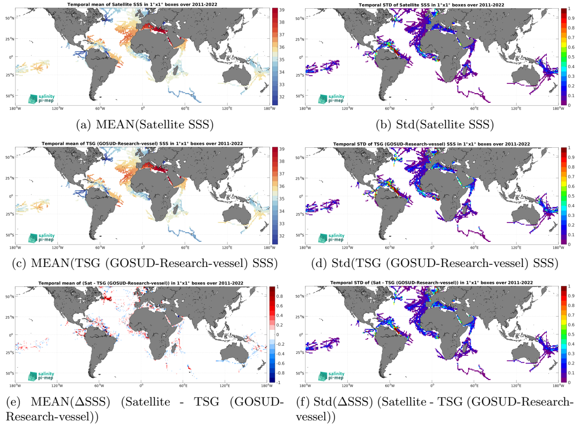
Figure 7: Temporal mean (left) and Std (right) of SSS from SMAP SSS L4 OI v3 - Daily (ESR) (top), TSG (GOSUD-Research-vessel) (middle), and of \Delta SSS (Satellite - TSG (GOSUD-Research-vessel)). Only match-up pairs are used to generate these maps.
