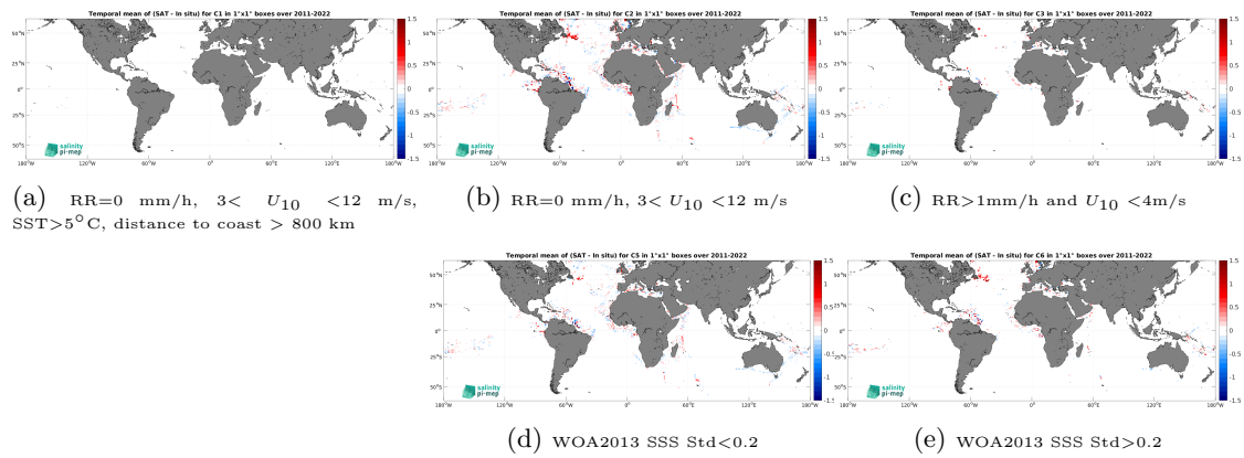
Figure 14: Temporal mean gridded over spatial boxes of size 1^\circ \times 1^\circ of \Delta\text{SSS} (SMAP SSS L4 OI v3 - Daily (ESR) - TSG (GOSUD-Research-vessel)) for 5 different subdatasets corresponding to:RR=0 mm/h, 3 < U_{10} < 12 m/s, SST>5°C, distance to coast > 800 km (a), RR=0 mm/h, 3 < U_{10} < 12 m/s (b), RR>1mm/h and U_{10} < 4 m/s (c), WOA2013 SSS Std<0.2 (d), WOA2013 SSS Std>0.2 (e).
