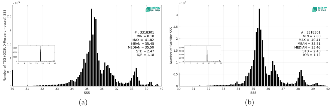
Figure 3: Histograms of SSS from TSG (GOSUD-Research-vessel) (a) and SMAP SSS L4 OI v3 - Daily (ESR) (b) considering all match-up pairs per bins of 0.1 over the SMOS coastal zone (<800km) 60N-60S Pi-MEP region and for the full satellite product period.
