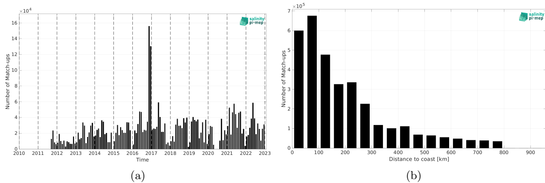
Figure 2: Number of match-ups between TSG (GOSUD-Research-vessel) and SMAP SSS L4 OI v3 - Daily (ESR) SSS as a function of time (a) and as function of the distance to coast (b) over the SMOS coastal zone (<800km) 60N-60S Pi-MEP region and for the full satellite product period.
