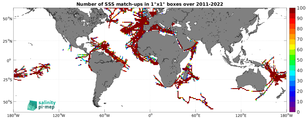
Figure 5: Number of SSS match-ups between TSG (GOSUD-Research-vessel) SSS and the SMAP SSS L4 OI v3 - Daily (ESR) SSS product for the SMOS coastal zone (<800km) 60N-60S Pi-MEP region over 1^{\circ} \times 1^{\circ} boxes and for the full satellite product period.
