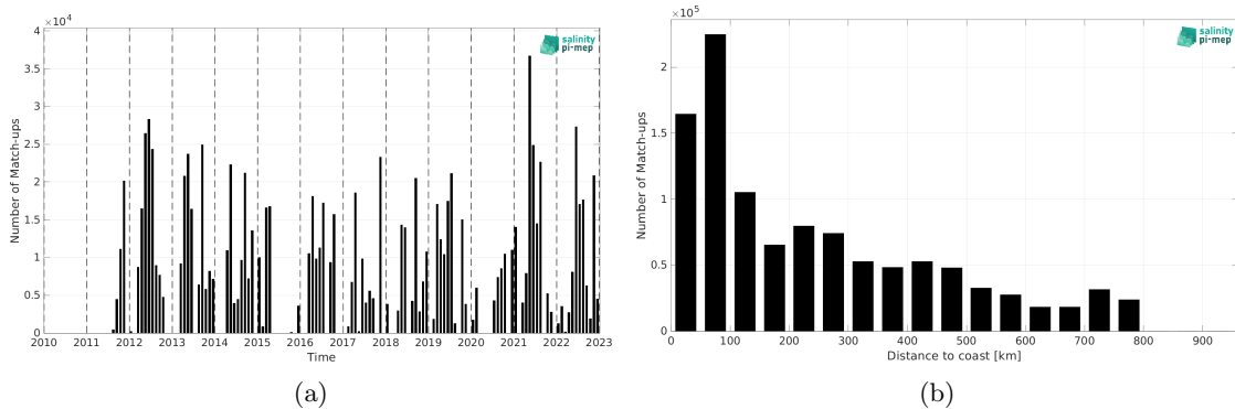
Figure 2: Number of match-ups between TSG (CSIC-UTM) and SMAP SSS L4 OI v3 - Daily (ESR) SSS as a function of time (a) and as function of the distance to coast (b) over the SMOS coastal zone (<800km) 60N-60S Pi-MEP region and for the full satellite product period.
