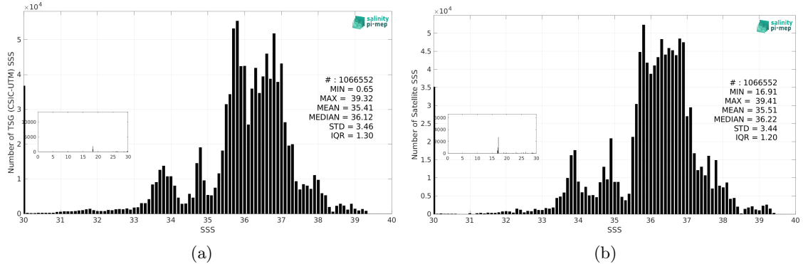
Figure 3: Histograms of SSS from TSG (CSIC-UTM) (a) and SMAP SSS L4 OI v3 - Daily (ESR) (b) considering all match-up pairs per bins of 0.1 over the SMOS coastal zone (<800km) 60N-60S Pi-MEP region and for the full satellite product period.
