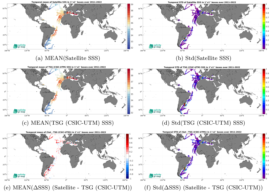
Figure 7: Temporal mean (left) and Std (right) of SSS from SMAP SSS L4 OI v3 - Daily (ESR) (top), TSG (CSIC-UTM) (middle), and of \Delta SSS (Satellite - TSG (CSIC-UTM)). Only match-up pairs are used to generate these maps.
