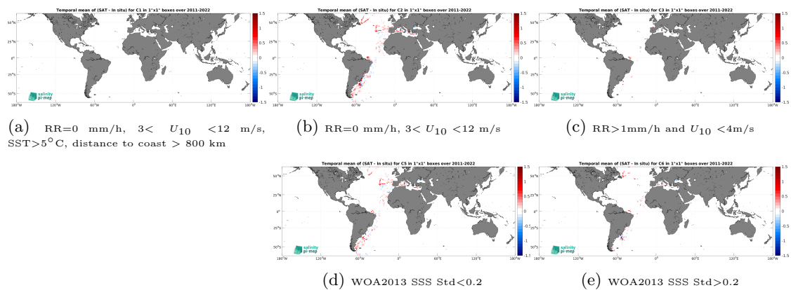
Figure 14: Temporal mean gridded over spatial boxes of size 1^\circ \times 1^\circ of \Delta SSS (SMAP SSS L4 OI v3 - Daily (ESR) - TSG (CSIC-UTM)) for 5 different subdatasets corresponding to: RR=0 mm/h, 3 < U_{10} < 12 m/s, SST > 5^\circ\text{C} , distance to coast > 800 km (a), RR=0 mm/h, 3 < U_{10} < 12 m/s (b), RR > 1 mm/h and U_{10} < 4 m/s (c), WOA2013 SSS Std < 0.2 (d), WOA2013 SSS Std > 0.2 (e).
