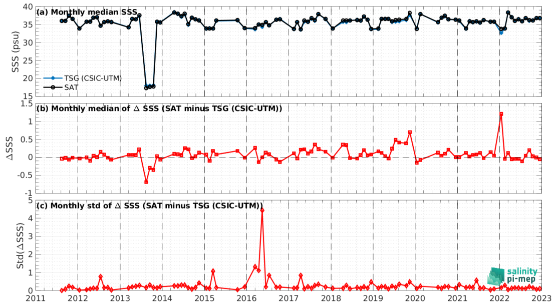
Figure 8: Time series of the monthly median SSS (top), median of \Delta SSS (Satellite - TSG (CSIC-UTM)) and Std of \Delta SSS (Satellite - TSG (CSIC-UTM)) over the SMOS coastal zone ( <800\text{km} ) 60\text{N} - 60\text{S} Pi-MEP region considering all match-ups collected by the Pi-MEP.
