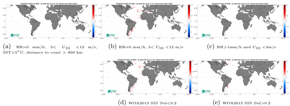
Figure 14: Temporal mean gridded over spatial boxes of size 1^\circ \times 1^\circ of \Delta SSS (SMAP SSS L4 OI v3 - Daily (ESR) - TSG (CSIC-UTM)) for 5 different subdatasets corresponding to:RR=0 mm/h, 3 < U_{10} < 12 m/s, SST >5^\circ\text{C} , distance to coast > 800 km (a), RR=0 mm/h, 3 < U_{10} < 12 m/s (b), RR >1 mm/h and U_{10} < 4 m/s (c), WOA2013 SSS Std <0.2 (d), WOA2013 SSS Std >0.2 (e).
