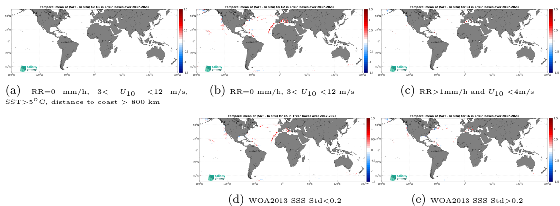
Figure 14: Temporal mean gridded over spatial boxes of size 1^\circ \times 1^\circ of \Delta SSS (SMAP SSS L4 OI v3 - Daily (ESR) - Saildrone) for 5 different subdatasets corresponding to:RR=0 mm/h, 3 < U_{10} < 12 m/s, SST >5^\circ\text{C} , distance to coast > 800 km (a), RR=0 mm/h, 3 < U_{10} < 12 m/s (b), RR >1 mm/h and U_{10} < 4 m/s (c), WOA2013 SSS Std <0.2 (d), WOA2013 SSS Std >0.2 (e).
