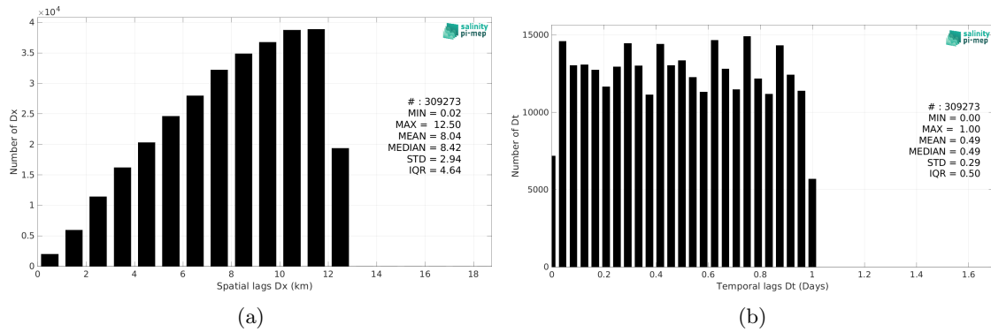
Figure 6: Histograms of the spatial (a) and temporal (b) lags between the location/time of the Sailability measurement and the date of the corresponding SMAP SSS L4 OI v3 - Daily (ESR) SSS pixel.
