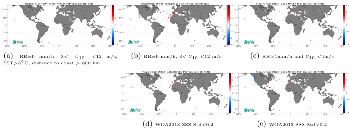
Figure 14: Temporal mean gridded over spatial boxes of size 1^\circ \times 1^\circ of \Delta\text{SSS} (SMAP SSS L4 OI v3 - Daily (ESR) - Saildrone) for 5 different subdatasets corresponding to:RR=0 mm/h, 3 < U_{10} < 12 m/s, SST>5°C, distance to coast > 800 km (a), RR=0 mm/h, 3 < U_{10} < 12 m/s (b), RR>1mm/h and U_{10} < 4 m/s (c), WOA2013 SSS Std<0.2 (d), WOA2013 SSS Std>0.2 (e).
