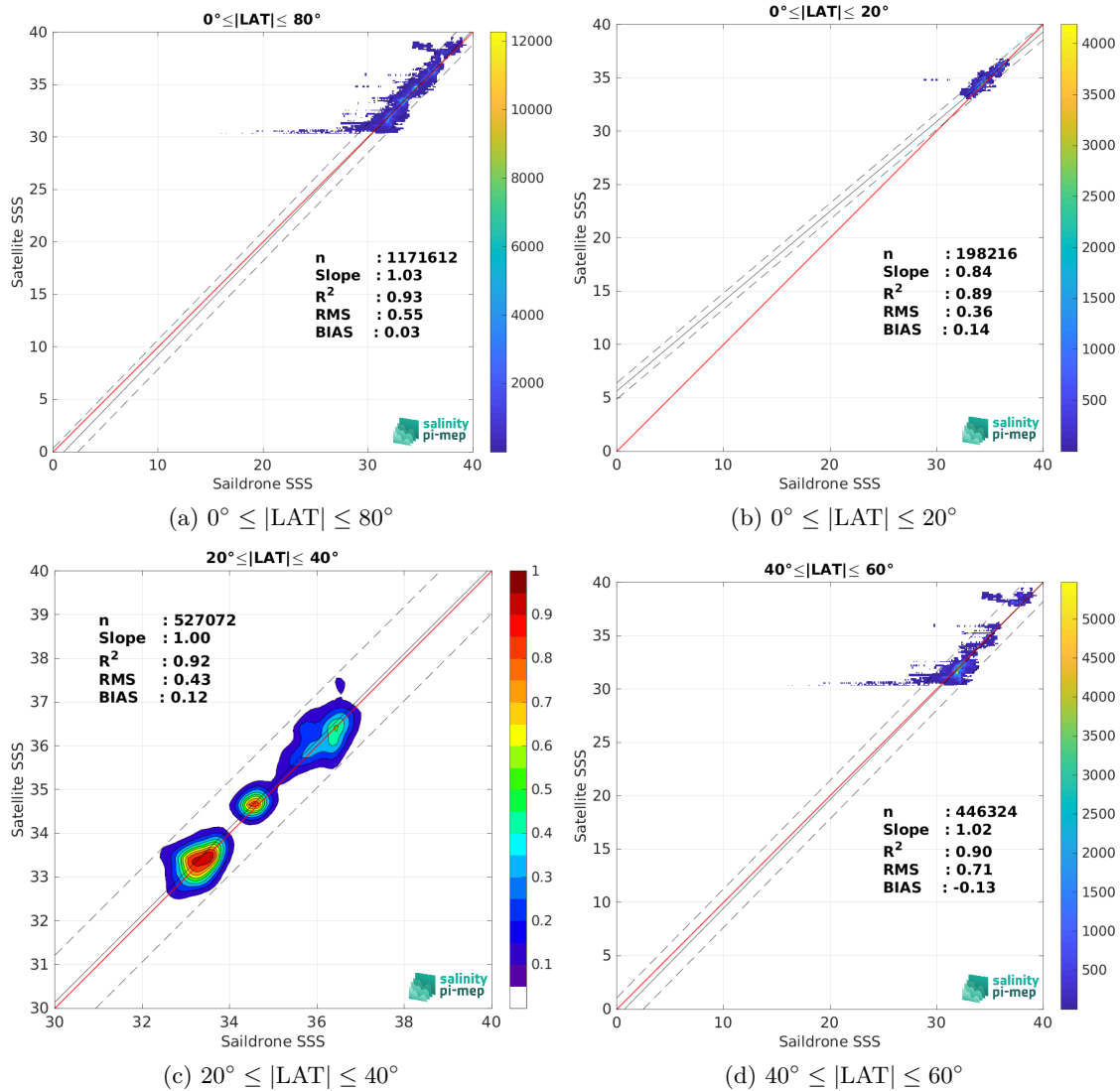
Figure 10: Contour maps of the concentration of SMAP SSS L4 OI v3 - Daily (ESR) SSS (y-axis) versus Saildrone SSS (x-axis) at match-up pairs for different latitude bands. For each plot, the red line shows x=y . The black thin and dashed lines indicate a linear fit through the data cloud and the \pm 95\% confidence levels, respectively. The number match-up pairs n , the slope and R^2 coefficient of the linear fit, the root mean square (RMS) and the mean bias between satellite and in situ data are indicated for each latitude band in each plots.
