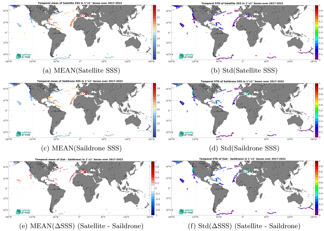
Figure 7: Temporal mean (left) and Std (right) of SSS from SMAP SSS L4 OI v3 - Daily (ESR) (top), Saildrone (middle), and of \Delta SSS (Satellite - Saildrone). Only match-up pairs are used to generate these maps.
