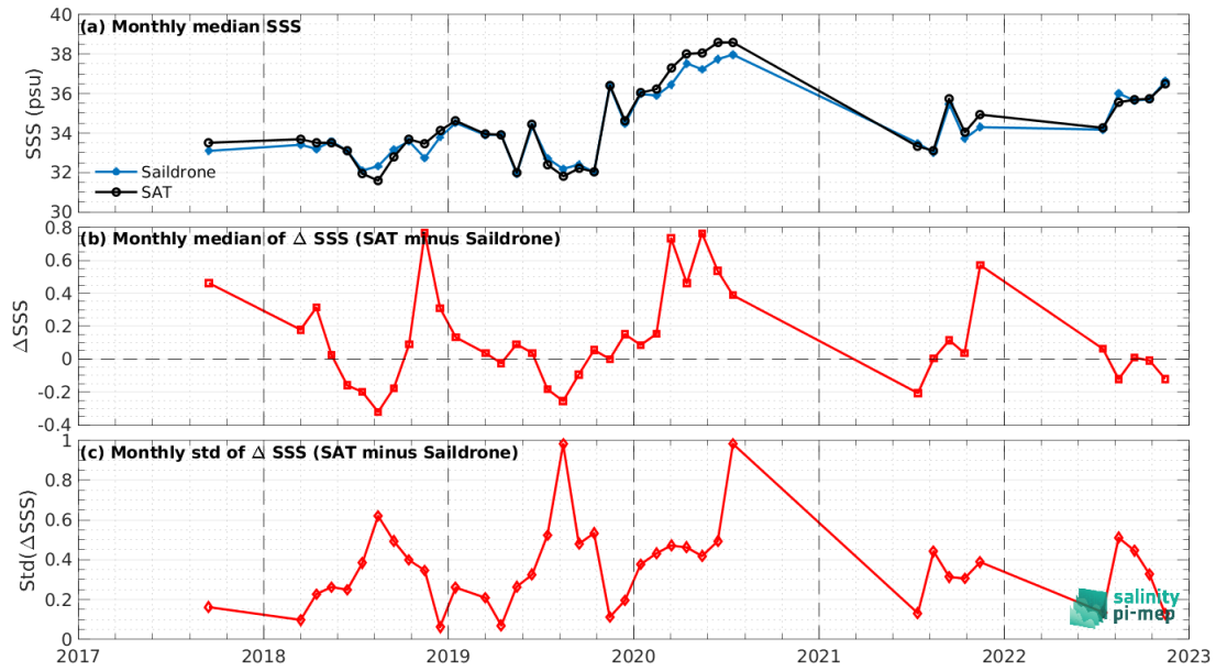
Figure 8: Time series of the monthly median SSS (top), median of \Delta SSS (Satellite - Saildrone) and Std of \Delta SSS (Satellite - Saildrone) over the SMOS coastal zone (<800km) 60N-60S Pi-MEP region considering all match-ups collected by the Pi-MEP.
