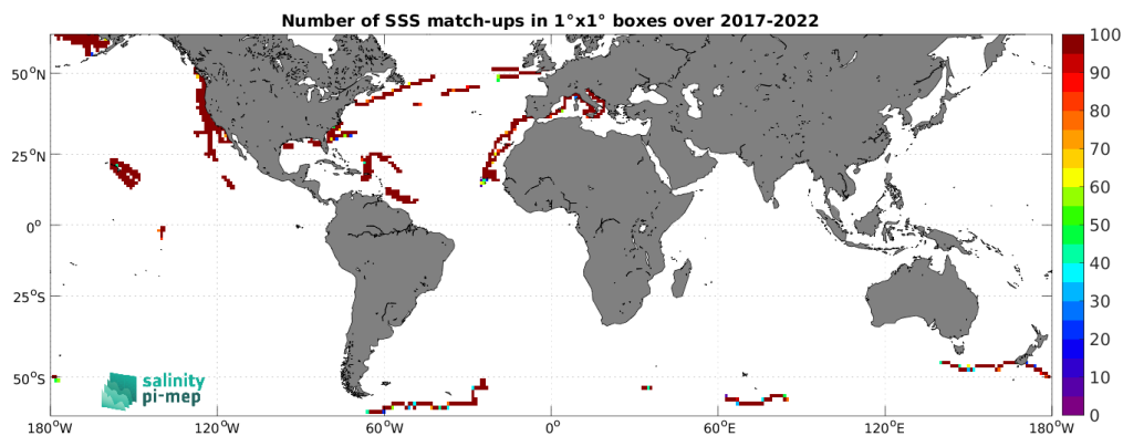
Figure 5: Number of SSS match-ups between Saildrone SSS and the SMAP SSS L4 OI v3 - Daily (ESR) SSS product for the SMOS coastal zone (<800km) 60N-60S Pi-MEP region over 1^\circ \times 1^\circ boxes and for the full satellite product period.
