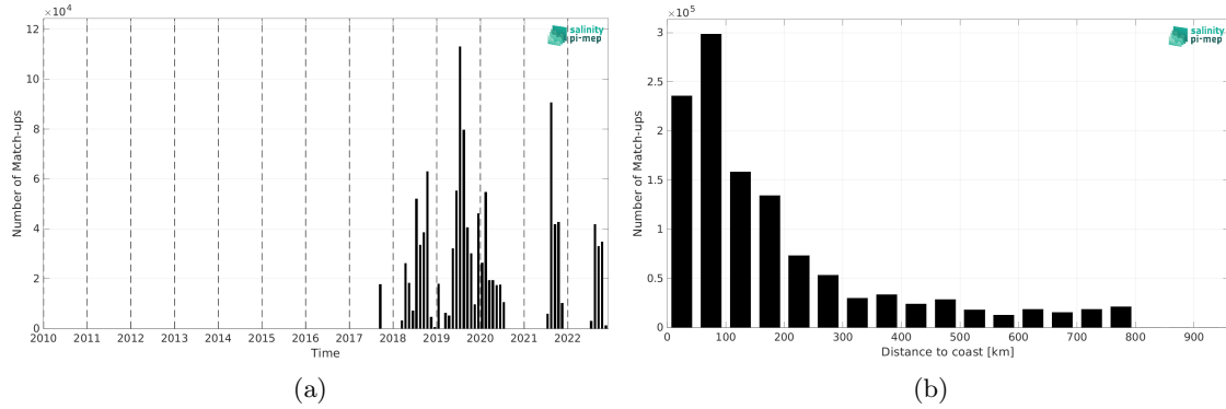
Figure 2: Number of match-ups between Saildrone and SMAP SSS L4 OI v3 - Daily (ESR) SSS as a function of time (a) and as function of the distance to coast (b) over the SMOS coastal zone (<800km) 60N-60S Pi-MEP region and for the full satellite product period.
