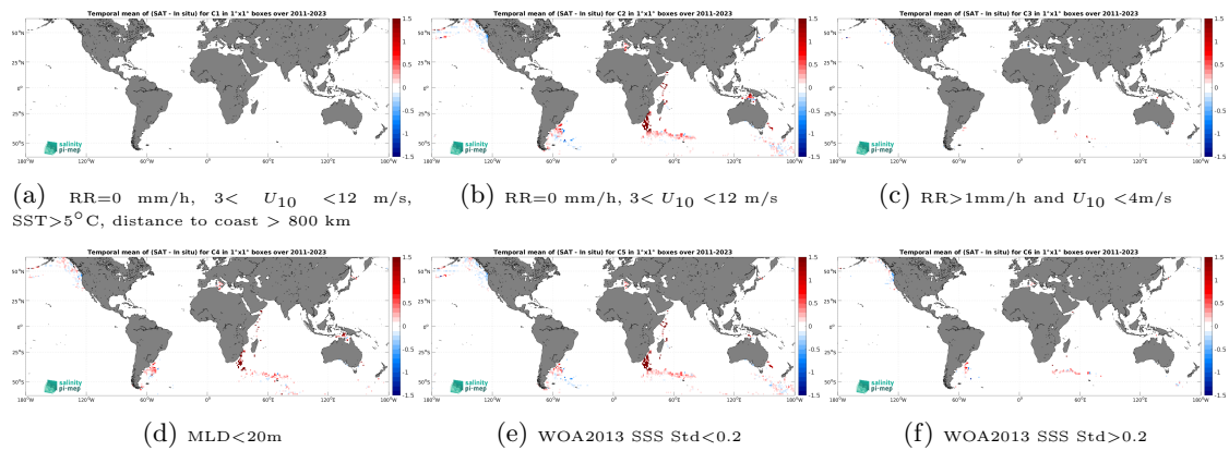
Figure 14: Temporal mean gridded over spatial boxes of size 1^\circ \times 1^\circ of \Delta SSS (SMAP SSS L4 OI v3 - Daily (ESR) - Marine mammals) for 6 different subdatasets corresponding to:RR=0 mm/h, 3 < U_{10} < 12 m/s, SST > 5^\circ\text{C} , distance to coast > 800 km (a), RR=0 mm/h, 3 < U_{10} < 12 m/s (b), RR > 1 mm/h and U_{10} < 4 m/s (c),MLD < 20 m (d),WOA2013 SSS Std < 0.2 (e),WOA2013 SSS Std > 0.2 (f).
