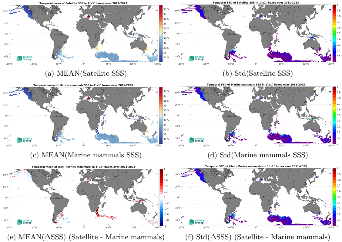
Figure 7: Temporal mean (left) and Std (right) of SSS from SMAP SSS L4 OI v3 - Daily (ESR) (top), Marine mammals (middle), and of \Delta SSS (Satellite - Marine mammals). Only match-up pairs are used to generate these maps.
