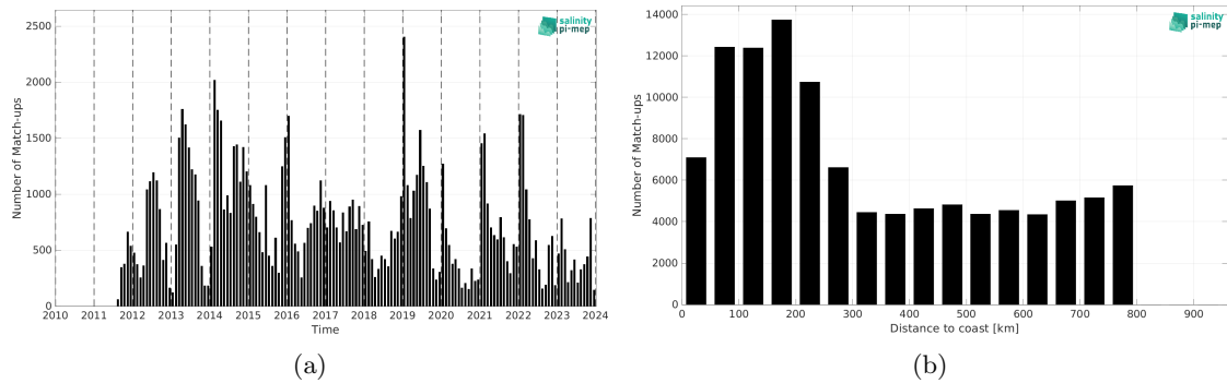
Figure 2: Number of match-ups between Marine mammals and SMAP SSS L4 OI v3 - Daily (ESR) SSS as a function of time (a) and as function of the distance to coast (b) over the SMOS coastal zone (<800km) 60N-60S Pi-MEP region and for the full satellite product period.
