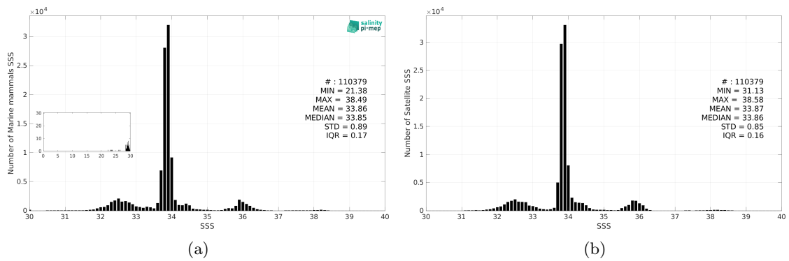
Figure 3: Histograms of SSS from Marine mammals (a) and SMAP SSS L4 OI v3 - Daily (ESR) (b) considering all match-up pairs per bins of 0.1 over the SMOS coastal zone (<800km) 60N-60S Pi-MEP region and for the full satellite product period.
