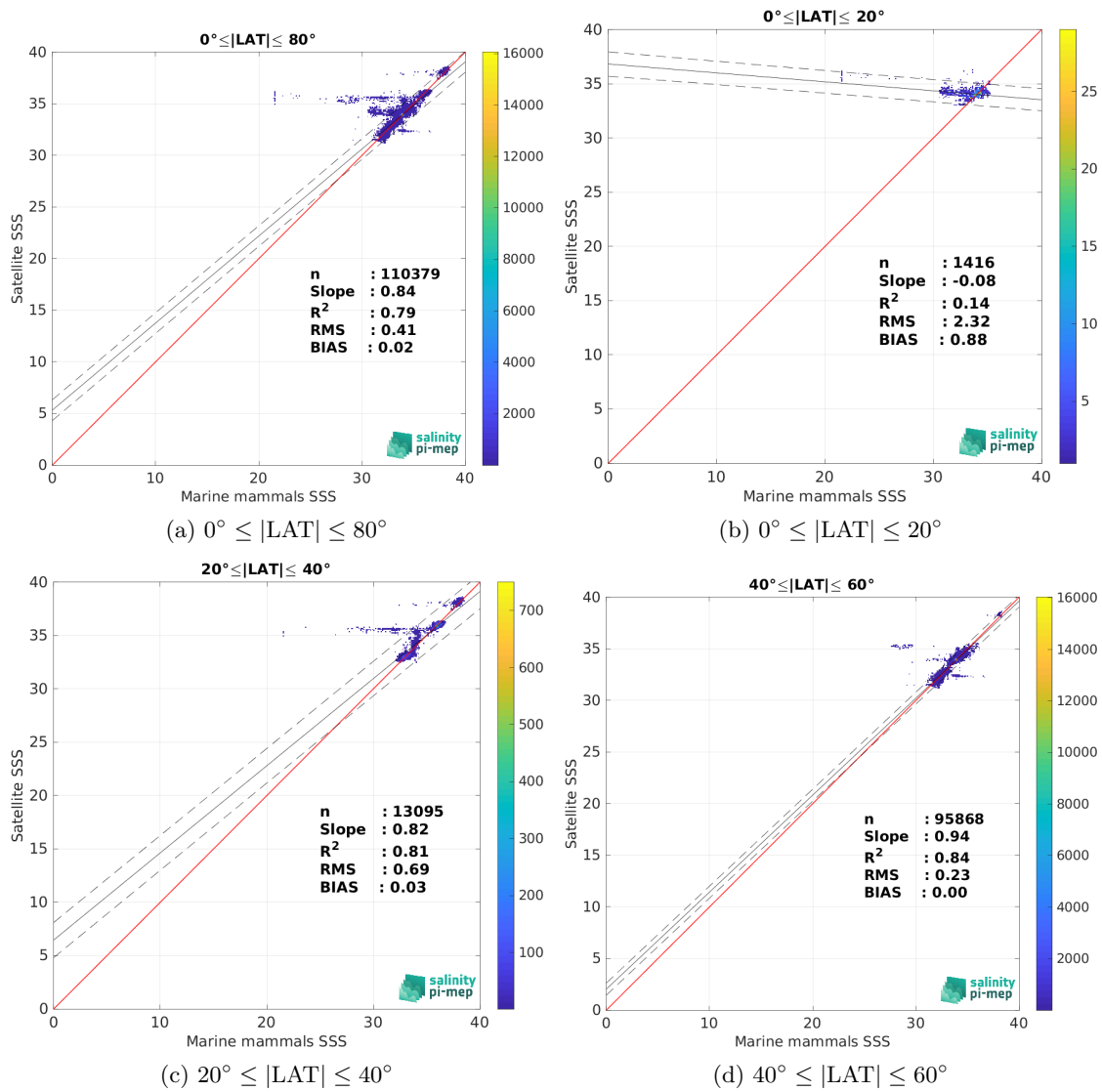
Figure 10: Contour maps of the concentration of SMAP SSS L4 OI v3 - Daily (ESR) SSS ( y -axis) versus Marine mammals SSS ( x -axis) at match-up pairs for different latitude bands. For each plot, the red line shows x=y . The black thin and dashed lines indicate a linear fit through the data cloud and the \pm 95\% confidence levels, respectively. The number match-up pairs n , the slope and R^2 coefficient of the linear fit, the root mean square (RMS) and the mean bias between satellite and in situ data are indicated for each latitude band in each plots.
