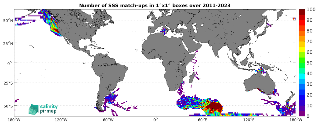
Figure 5: Number of SSS match-ups between Marine mammals SSS and the SMAP SSS L4 OI v3 - Daily (ESR) SSS product for the SMOS coastal zone (<800km) 60N-60S Pi-MEP region over 1^\circ \times 1^\circ boxes and for the full satellite product period.
