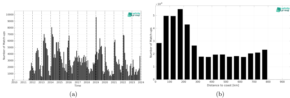
Figure 2: Number of match-ups between Marine mammals and SMAP SSS L4 OI v3 - Daily (ESR) SSS as a function of time (a) and as function of the distance to coast (b) over the SMOS coastal zone (<800km) 60N-60S Pi-MEP region and for the full satellite product period.
