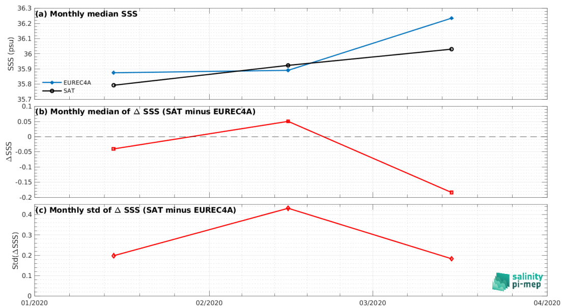
Figure 8: Time series of the monthly median SSS (top), median of \Delta SSS (Satellite - EUREC4A) and Std of \Delta SSS (Satellite - EUREC4A) over the SMOS coastal zone (<800km) 60N-60S Pi-MEP region considering all match-ups collected by the Pi-MEP.
