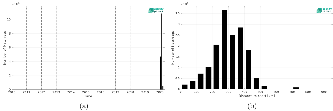
Figure 2: Number of match-ups between EUREC4A and SMAP SSS L4 OI v3 - Daily (ESR) SSS as a function of time (a) and as function of the distance to coast (b) over the SMOS coastal zone (<800km) 60N-60S Pi-MEP region and for the full satellite product period.
