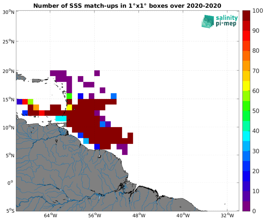
Figure 5: Number of SSS match-ups between EUREC4A SSS and the SMAP SSS L4 OI v3 - Daily (ESR) SSS product for the SMOS coastal zone (<800km) 60N-60S Pi-MEP region over 1^{\circ} \times 1^{\circ} boxes and for the full satellite product period.
