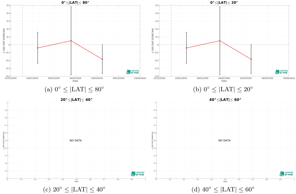
Figure 11: Monthly median (red curves) of \Delta SSS (Satellite - EUREC4A) and \pm 1 Std (black vertical thick bars) as function of time for all the collected Pi-MEP match-up pairs estimated over the SMOS coastal zone (<800km) 60N-60S Pi-MEP region and for the full satellite product period are shown for different latitude bands: (a) 80°S-80°N, (b) 20°S-20°N, (c) 40°S-20°S and 20°N-40°N and (d) 60°S-40°S and 40°N-60°N.
