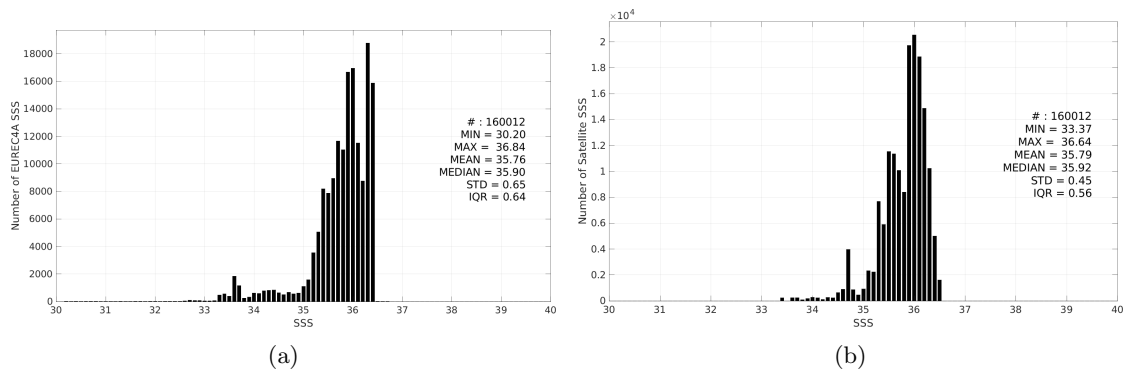
Figure 3: Histograms of SSS from EUREC4A (a) and SMAP SSS L4 OI v3 - Daily (ESR) (b) considering all match-up pairs per bins of 0.1 over the SMOS coastal zone (<800km) 60N-60S Pi-MEP region and for the full satellite product period.
