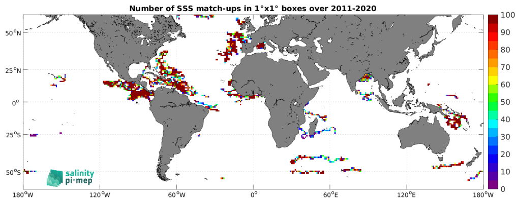
Figure 4: Number of SSS match-ups between Surface drifters SSS and the SMAP SSS L4 OI v3 - Daily (ESR) SSS product for the SMOS coastal zone (<800km) 60N-60S Pi-MEP region over 1^\circ \times 1^\circ boxes and for the full satellite product period.
