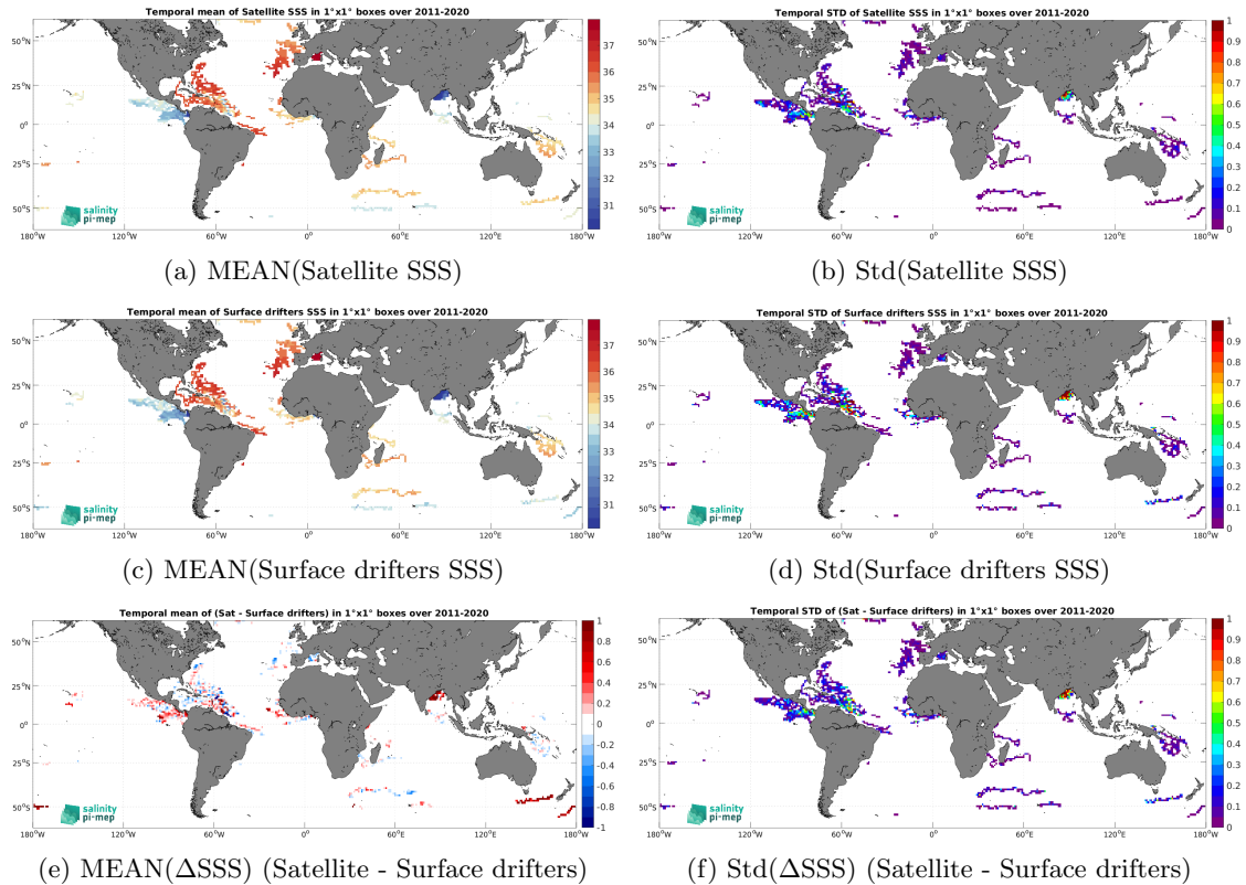
Figure 6: Temporal mean (left) and Std (right) of SSS from SMAP SSS L4 OI v3 - Daily (ESR) (top), Surface drifters (middle), and of \Delta SSS (Satellite - Surface drifters). Only match-up pairs are used to generate these maps.
