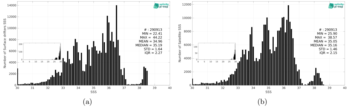
Figure 3: Histograms of SSS from Surface drifters (a) and SMAP SSS L4 OI v3 - Daily (ESR) (b) considering all match-up pairs per bins of 0.1 over the SMOS coastal zone (<800km) 60N-60S Pi-MEP region and for the full satellite product period.
