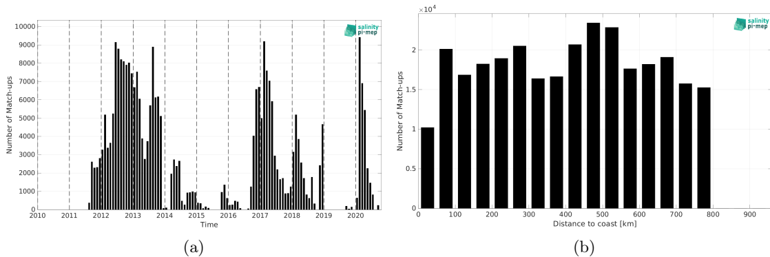
Figure 2: Number of match-ups between Surface drifters and SMAP SSS L4 OI v3 - Daily (ESR) SSS as a function of time (a) and as function of the distance to coast (b) over the SMOS coastal zone ( < 800\text{km} ) 60N-60S Pi-MEP region and for the full satellite product period.
