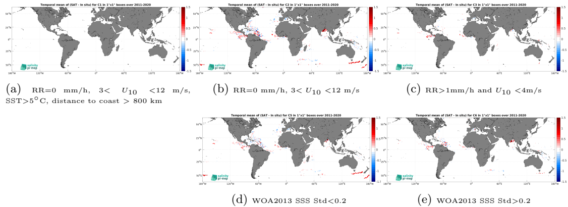
Figure 13: Temporal mean gridded over spatial boxes of size 1^\circ \times 1^\circ of \Delta\text{SSS} (SMAP SSS L4 OI v3 - Daily (ESR) - Surface drifters) for 5 different subdatasets corresponding to:RR=0 mm/h, 3 < U_{10} < 12 m/s, SST >5^\circ\text{C} , distance to coast > 800 km (a), RR=0 mm/h, 3 < U_{10} < 12 m/s (b), RR >1 mm/h and U_{10} < 4 m/s (c), WOA2013 SSS Std <0.2 (d), WOA2013 SSS Std >0.2 (e).
