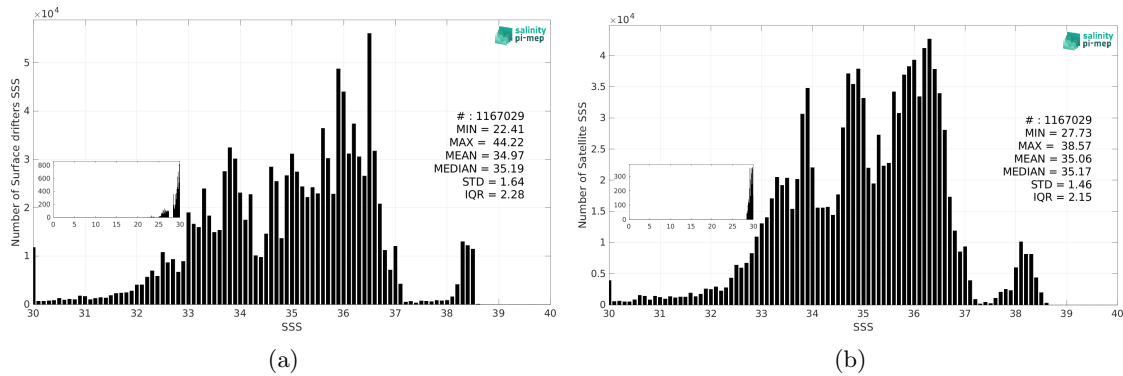
Figure 3: Histograms of SSS from Surface drifters (a) and SMAP SSS L4 OI v3 - Daily (ESR) (b) considering all match-up pairs per bins of 0.1 over the SMOS coastal zone ( <800\text{km} ) 60N-60S Pi-MEP region and for the full satellite product period.
