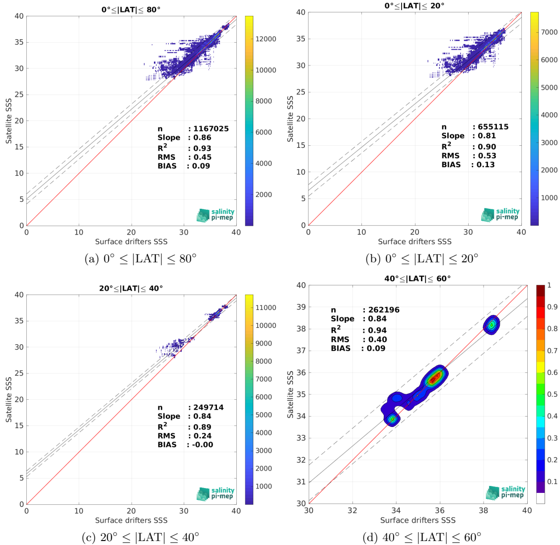
Figure 9: Contour maps of the concentration of SMAP SSS L4 OI v3 - Daily (ESR) SSS (y-axis) versus Surface drifters SSS (x-axis) at match-up pairs for different latitude bands. For each plot, the red line shows x=y . The black thin and dashed lines indicate a linear fit through the data cloud and the \pm 95\% confidence levels, respectively. The number match-up pairs n , the slope and R^2 coefficient of the linear fit, the root mean square (RMS) and the mean bias between satellite and in situ data are indicated for each latitude band in each plots.
