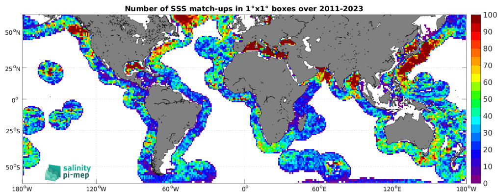
Figure 5: Number of SSS match-ups between Argo SSS and the SMAP SSS L4 OI v3 - Daily (ESR) SSS product for the SMOS coastal zone (<800km) 60N-60S Pi-MEP region over 1^\circ \times 1^\circ boxes and for the full satellite product period.
