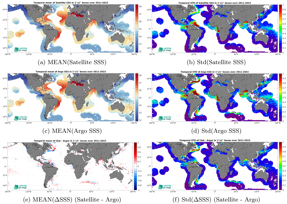
Figure 7: Temporal mean (left) and Std (right) of SSS from SMAP SSS L4 OI v3 - Daily (ESR) (top), Argo (middle), and of \Delta SSS (Satellite - Argo). Only match-up pairs are used to generate these maps.
