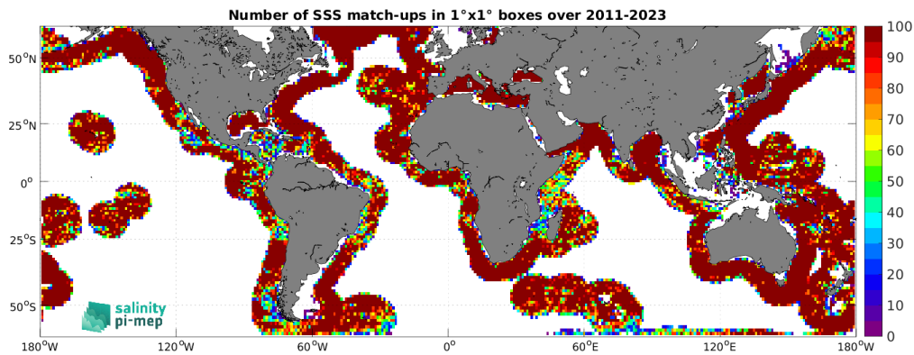
Figure 5: Number of SSS match-ups between Argo SSS and the SMAP SSS L4 OI v3 - Daily (ESR) SSS product for the SMOS coastal zone ( <800\text{km} ) 60N-60S Pi-MEP region over 1^\circ \times 1^\circ boxes and for the full satellite product period.
