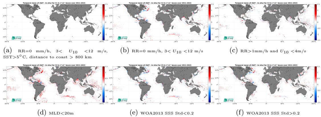
Figure 14: Temporal mean gridded over spatial boxes of size 1^\circ \times 1^\circ of \Delta SSS (SMAP SSS L4 OI v3 - Daily (ESR) - Argo) for 6 different subdatasets corresponding to:RR=0 mm/h, 3 < U_{10} < 12 m/s, SST >5^\circ C, distance to coast > 800 km (a), RR=0 mm/h, 3 < U_{10} < 12 m/s (b), RR >1 mm/h and U_{10} < 4 m/s (c),MLD <20 m (d),WOA2013 SSS Std <0.2 (e),WOA2013 SSS Std >0.2 (f).
