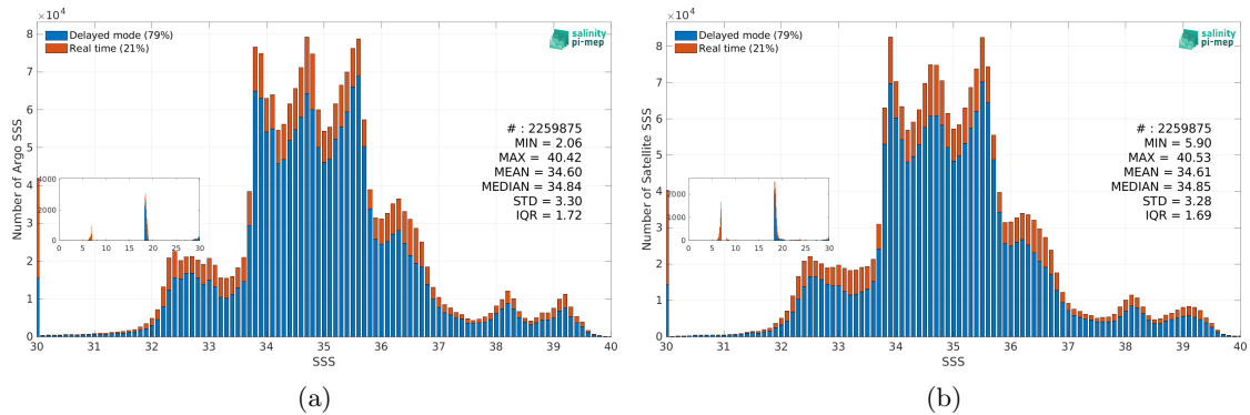
Figure 3: Histograms of SSS from Argo (a) and SMAP SSS L4 OI v3 - Daily (ESR) (b) considering all match-up pairs per bins of 0.1 over the SMOS coastal zone (<800km) 60N-60S Pi-MEP region and for the full satellite product period.
