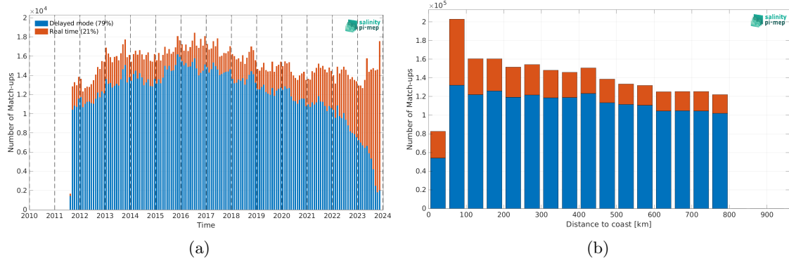
Figure 2: Number of match-ups between Argo and SMAP SSS L4 OI v3 - Daily (ESR) SSS as a function of time (a) and as function of the distance to coast (b) over the SMOS coastal zone (<800km) 60N-60S Pi-MEP region and for the full satellite product period.
