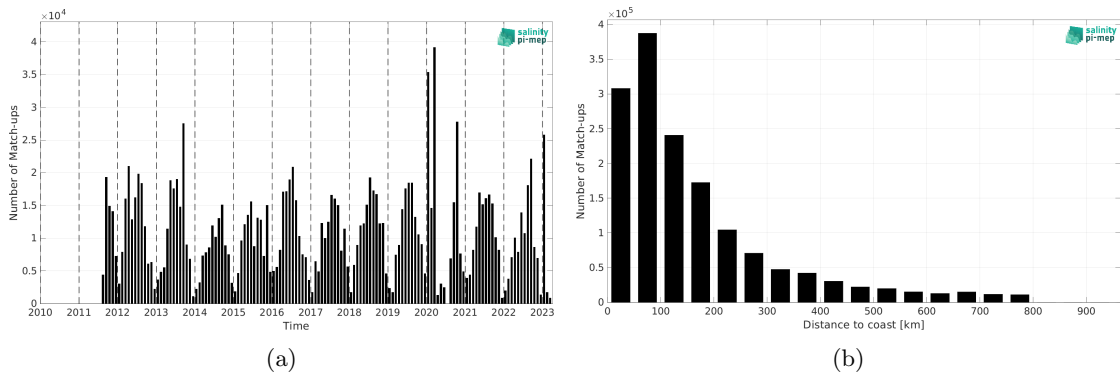
Figure 1: Number of match-ups between TSG (SAMOS) and SMAP SSS L4 OI v2 - 7 Days (ESR) SSS as a function of time (a) and as function of the distance to coast (b) over the SMOS coastal zone ( < 800\text{km} ) 60N-60S Pi-MEP region and for the full satellite product period.
