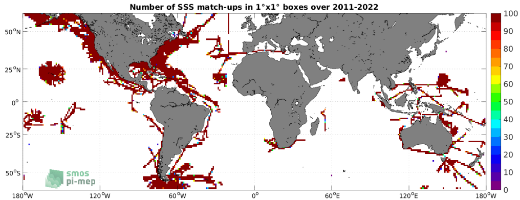
Figure 4: Number of SSS match-ups between TSG (SAMOS) SSS and the SMAP SSS L4 OI v2 - 7 Days (ESR) SSS product for the SMOS coastal zone (<800km) 60N-60S Pi-MEP region over 1^\circ \times 1^\circ boxes and for the full satellite product period.
