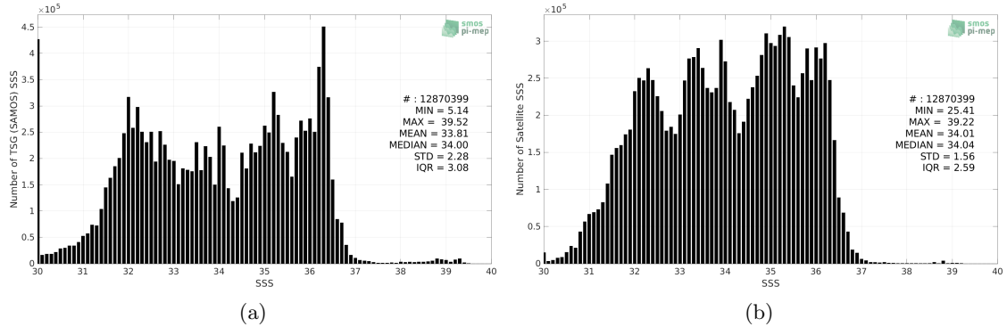
Figure 2: Histograms of SSS from TSG (SAMOS) (a) and SMAP SSS L4 OI v2 - 7 Days (ESR) (b) considering all match-up pairs per bins of 0.1 over the SMOS coastal zone (<800km) 60N-60S Pi-MEP region and for the full satellite product period.
