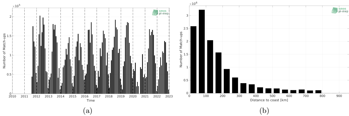
Figure 1: Number of match-ups between TSG (SAMOS) and SMAP SSS L4 OI v2 - 7 Days (ESR) SSS as a function of time (a) and as function of the distance to coast (b) over the SMOS coastal zone (<800km) 60N-60S Pi-MEP region and for the full satellite product period.
