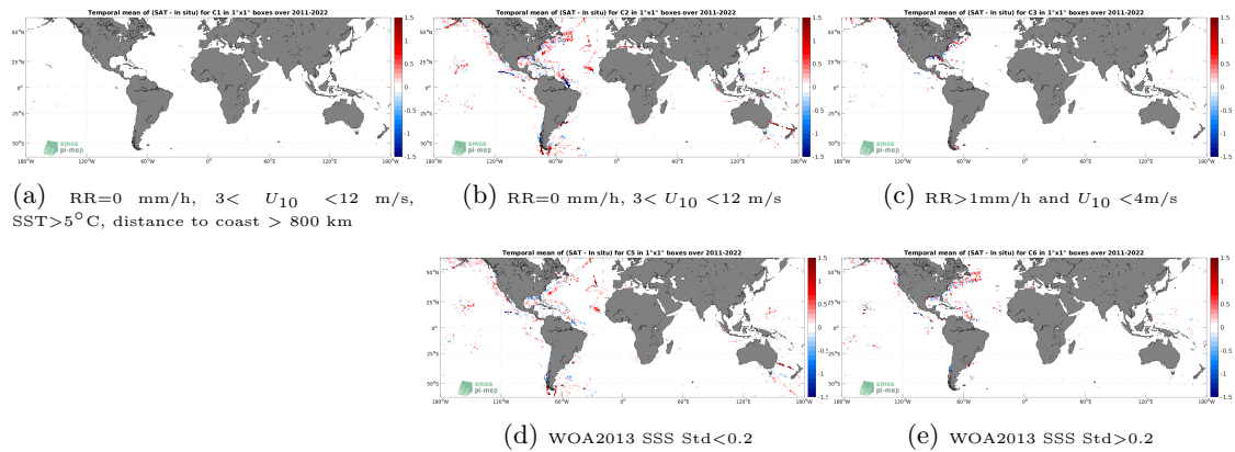
Figure 12: Temporal mean gridded over spatial boxes of size 1^\circ \times 1^\circ of \Delta SSS (SMAP SSS L4 OI v2 - 7 Days (ESR) - TSG (SAMOS)) for 5 different subdatasets corresponding to:RR=0 mm/h, 3 < U_{10} < 12 m/s, SST >5^\circ\text{C} , distance to coast > 800 km (a), RR=0 mm/h, 3 < U_{10} < 12 m/s (b), RR >1 mm/h and U_{10} < 4 m/s (c), WOA2013 SSS Std <0.2 (d), WOA2013 SSS Std >0.2 (e).
