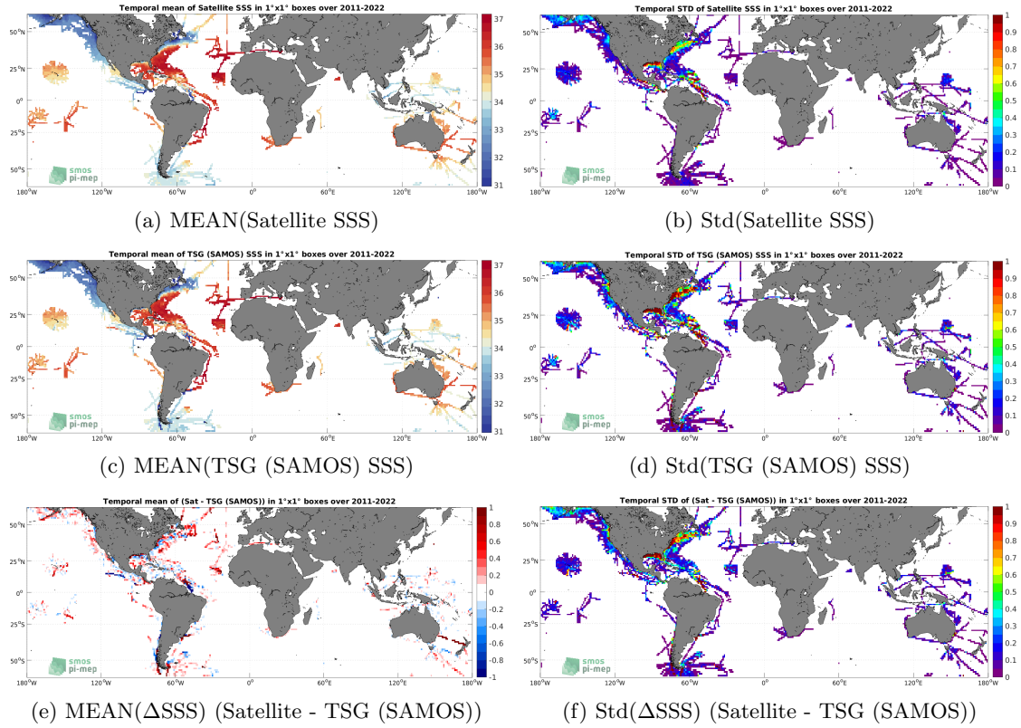
Figure 6: Temporal mean (left) and Std (right) of SSS from SMAP SSS L4 OI v2 - 7 Days (ESR) (top), TSG (SAMOS) (middle), and of \Delta SSS (Satellite - TSG (SAMOS)). Only match-up pairs are used to generate these maps.
