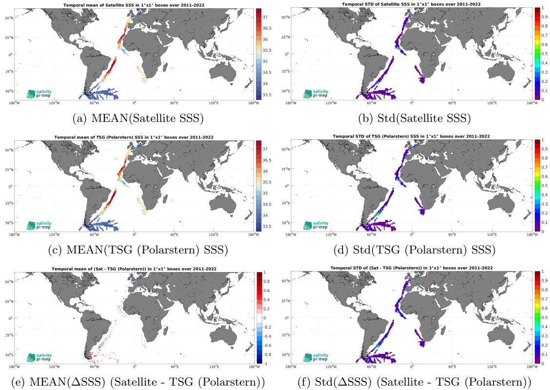
Figure 6: Temporal mean (left) and Std (right) of SSS from SMAP SSS L4 OI v2 - 7 Days (ESR) (top), TSG (Polarstern) (middle), and of \Delta SSS (Satellite - TSG (Polarstern)). Only match-up pairs are used to generate these maps.
