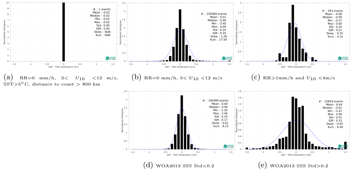
Figure 13: Normalized histogram of \Delta SSS (SMAP SSS L4 OI v2 - 7 Days (ESR) - TSG (Polarstern)) for 5 different subdatasets corresponding to: RR=0 mm/h, 3 < U_{10} < 12 m/s, SST > 5°C, distance to coast > 800 km (a), RR=0 mm/h, 3 < U_{10} < 12 m/s (b), RR > 1mm/h and U_{10} < 4 m/s (c), WOA2013 SSS Std < 0.2 (d), WOA2013 SSS Std > 0.2 (e).
