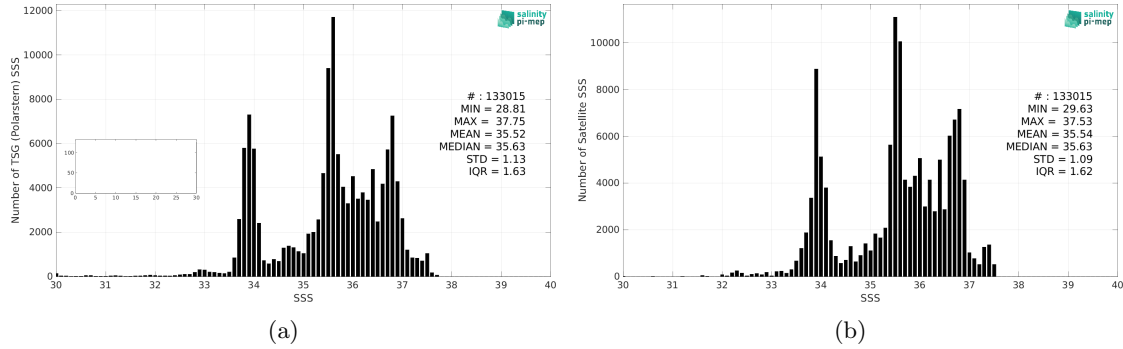
Figure 2: Histograms of SSS from TSG (Polarstern) (a) and SMAP SSS L4 OI v2 - 7 Days (ESR) (b) considering all match-up pairs per bins of 0.1 over the SMOS coastal zone (<800km) 60N-60S Pi-MEP region and for the full satellite product period.
