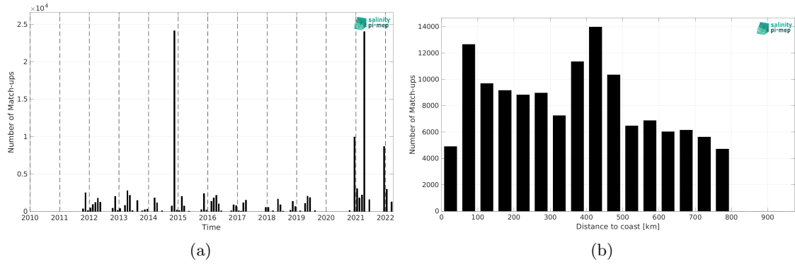
Figure 1: Number of match-ups between TSG (Polarstern) and SMAP SSS L4 OI v2 - 7 Days (ESR) SSS as a function of time (a) and as function of the distance to coast (b) over the SMOS coastal zone (<800km) 60N-60S Pi-MEP region and for the full satellite product period.
