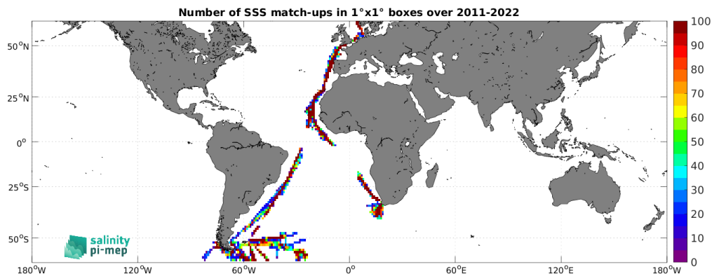
Figure 4: Number of SSS match-ups between TSG (Polarstern) SSS and the SMAP SSS L4 OI v2 - 7 Days (ESR) SSS product for the SMOS coastal zone (<800km) 60N-60S Pi-MEP region over 1^\circ \times 1^\circ boxes and for the full satellite product period.
