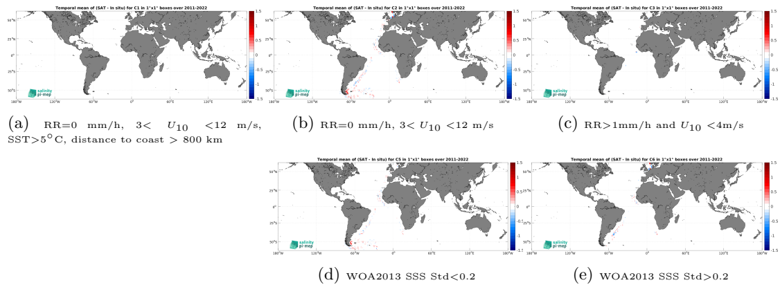
Figure 12: Temporal mean gridded over spatial boxes of size 1^\circ \times 1^\circ of \Delta SSS (SMAP SSS L4 OI v2 - 7 Days (ESR) - TSG (Polarstern)) for 5 different subdatasets corresponding to:RR=0 mm/h, 3 < U_{10} < 12 m/s, SST >5^\circ C, distance to coast > 800 km (a), RR=0 mm/h, 3 < U_{10} < 12 m/s (b), RR >1 mm/h and U_{10} < 4 m/s (c), WOA2013 SSS Std <0.2 (d), WOA2013 SSS Std >0.2 (e).
