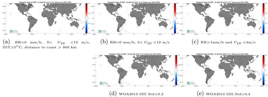
Figure 12: Temporal mean gridded over spatial boxes of size 1^\circ \times 1^\circ of \Delta SSS (SMAP SSS L4 OI v2 - 7 Days (ESR) - TSG (Polarstern)) for 5 different subdatasets corresponding to: RR=0 mm/h, 3 < U_{10} < 12 m/s, SST > 5^\circ C , distance to coast > 800 km (a), RR=0 mm/h, 3 < U_{10} < 12 m/s (b), RR > 1 mm/h and U_{10} < 4 m/s (c), WOA2013 SSS Std < 0.2 (d), WOA2013 SSS Std > 0.2 (e).
