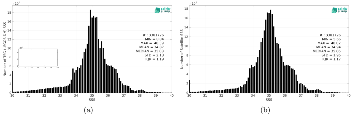
Figure 2: Histograms of SSS from TSG (LEGOS-DM) (a) and SMAP SSS L4 OI v2 - 7 Days (ESR) (b) considering all match-up pairs per bins of 0.1 over the SMOS coastal zone (<800km) 60N-60S Pi-MEP region and for the full satellite product period.
