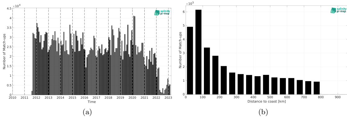
Figure 1: Number of match-ups between TSG (LEGOS-DM) and SMAP SSS L4 OI v2 - 7 Days (ESR) SSS as a function of time (a) and as function of the distance to coast (b) over the SMOS coastal zone (<800km) 60N-60S Pi-MEP region and for the full satellite product period.
