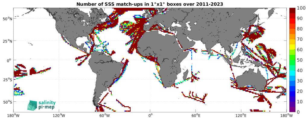
Figure 4: Number of SSS match-ups between TSG (LEGOS-DM) SSS and the SMAP SSS L4 OI v2 - 7 Days (ESR) SSS product for the SMOS coastal zone (<800km) 60N-60S Pi-MEP region over 1^\circ \times 1^\circ boxes and for the full satellite product period.
