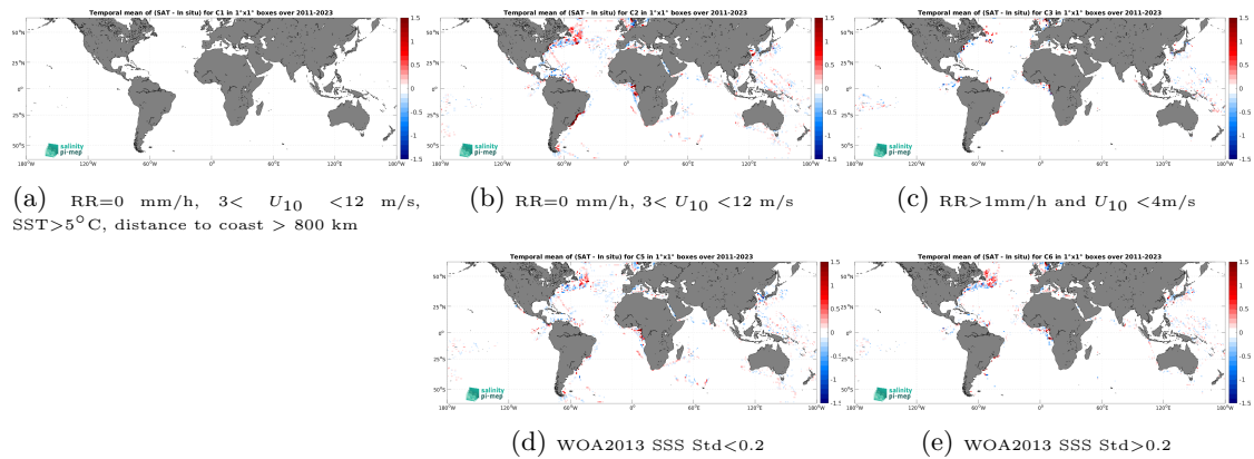
Figure 12: Temporal mean gridded over spatial boxes of size 1^\circ \times 1^\circ of \Delta\text{SSS} (SMAP SSS L4 OI v2 - 7 Days (ESR) - TSG (LEGOS-DM)) for 5 different subdatasets corresponding to:RR=0 mm/h, 3 < U_{10} < 12 m/s, SST >5^\circ\text{C} , distance to coast > 800 km (a), RR=0 mm/h, 3 < U_{10} < 12 m/s (b), RR >1 mm/h and U_{10} < 4 m/s (c), WOA2013 SSS Std <0.2 (d), WOA2013 SSS Std >0.2 (e).
