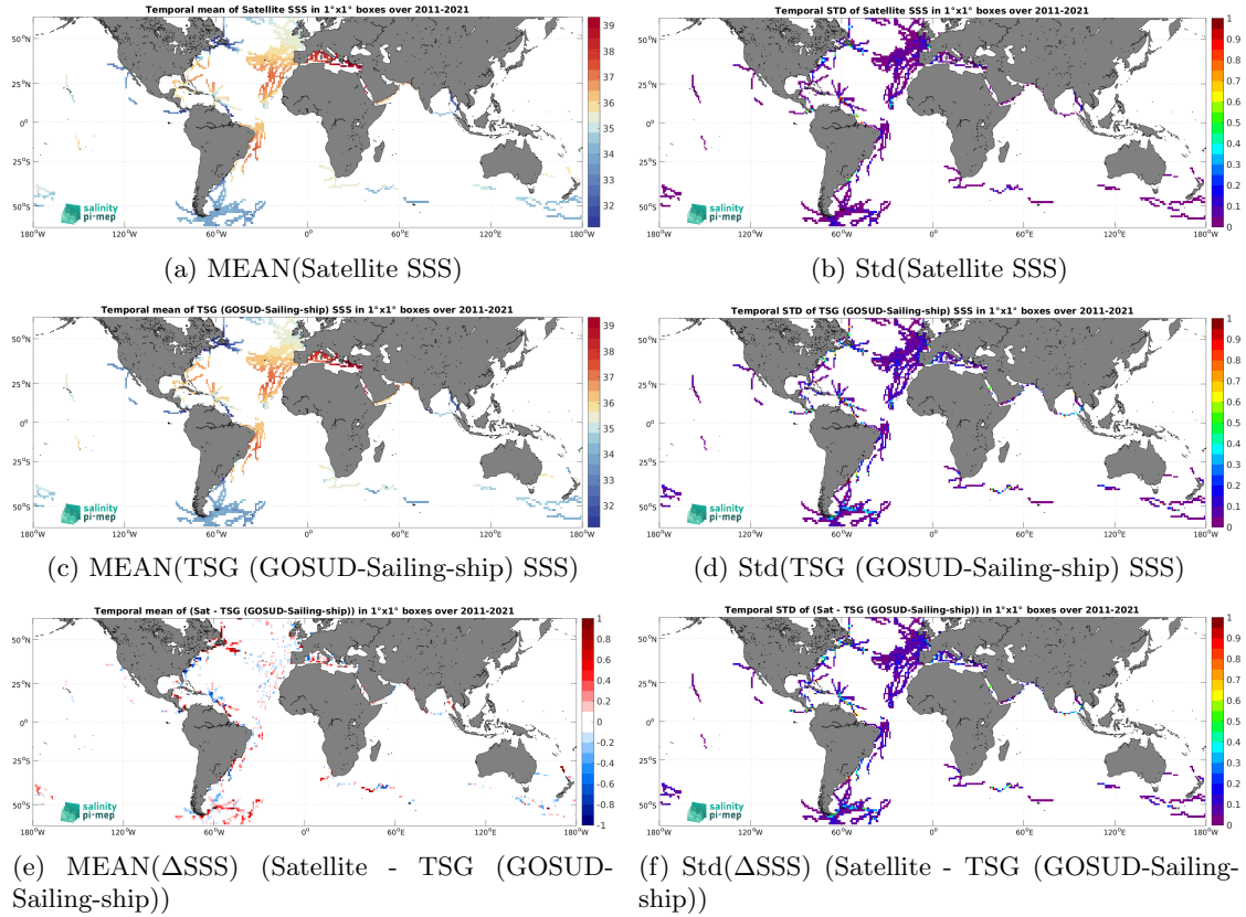
Figure 6: Temporal mean (left) and Std (right) of SSS from SMAP SSS L4 OI v2 - 7 Days (ESR) (top), TSG (GOSUD-Sailing-ship) (middle), and of \Delta SSS (Satellite - TSG (GOSUD-Sailing-ship)). Only match-up pairs are used to generate these maps.
