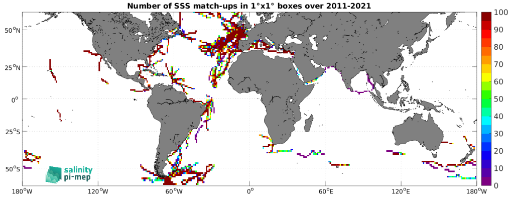
Figure 4: Number of SSS match-ups between TSG (GOSUD-Sailing-ship) SSS and the SMAP SSS L4 OI v2 - 7 Days (ESR) SSS product for the SMOS coastal zone (<800km) 60N-60S Pi-MEP region over 1^\circ \times 1^\circ boxes and for the full satellite product period.
