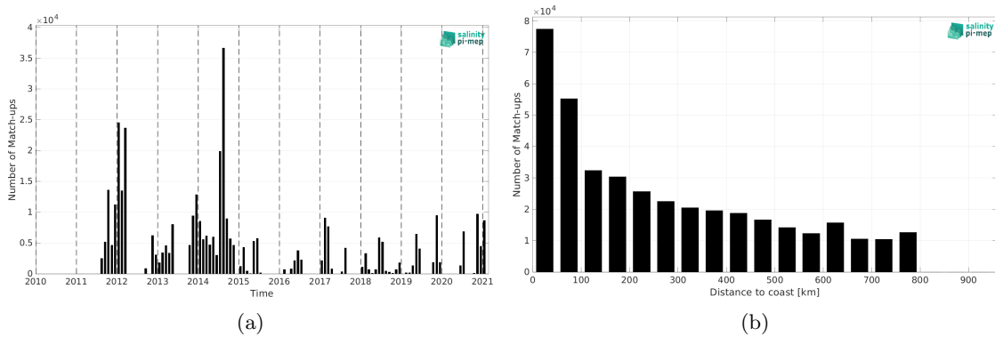
Figure 1: Number of match-ups between TSG (GOSUD-Sailing-ship) and SMAP SSS L4 OI v2 - 7 Days (ESR) SSS as a function of time (a) and as function of the distance to coast (b) over the SMOS coastal zone (<800km) 60N-60S Pi-MEP region and for the full satellite product period.
