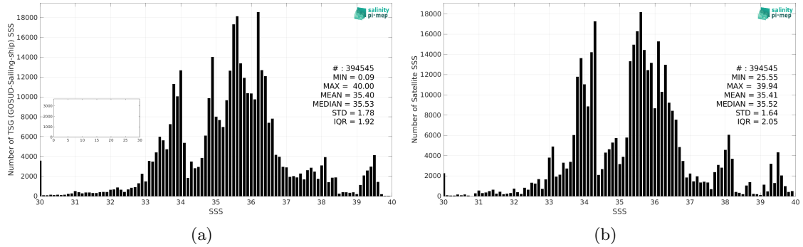
Figure 2: Histograms of SSS from TSG (GOSUD-Sailing-ship) (a) and SMAP SSS L4 OI v2 - 7 Days (ESR) (b) considering all match-up pairs per bins of 0.1 over the SMOS coastal zone (<800km) 60N-60S Pi-MEP region and for the full satellite product period.
