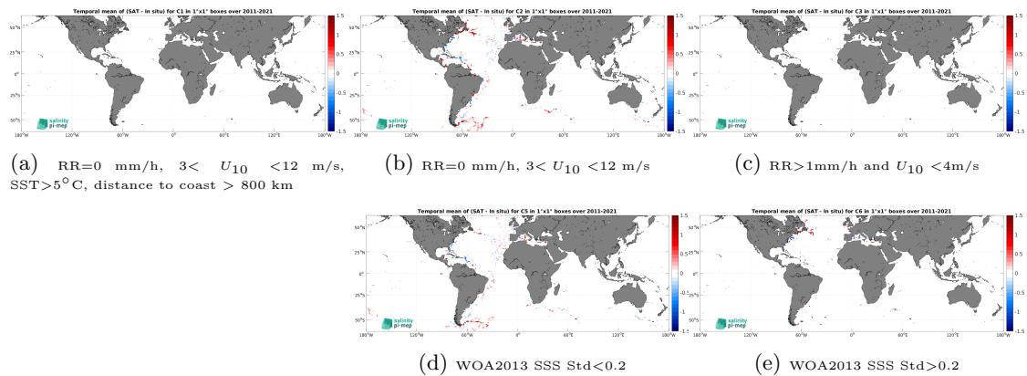
Figure 12: Temporal mean gridded over spatial boxes of size 1^\circ \times 1^\circ of \Delta\text{SSS} (SMAP SSS L4 OI v2 - 7 Days (ESR) - TSG (GOSUD-Sailing-ship)) for 5 different subdatasets corresponding to:RR=0 mm/h, 3 < U_{10} < 12 m/s, SST > 5^\circ\text{C} , distance to coast > 800 km (a), RR=0 mm/h, 3 < U_{10} < 12 m/s (b), RR > 1 mm/h and U_{10} < 4 m/s (c), WOA2013 SSS Std < 0.2 (d), WOA2013 SSS Std > 0.2 (e).
