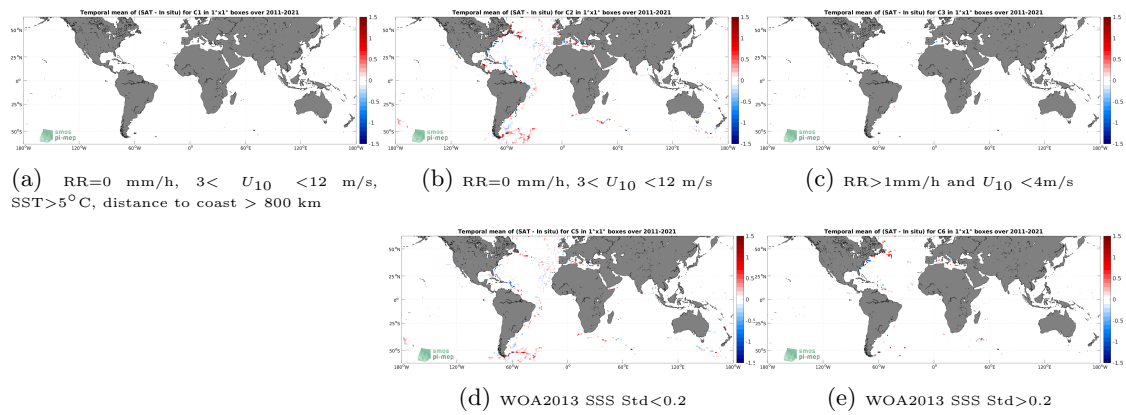
Figure 12: Temporal mean gridded over spatial boxes of size 1^\circ \times 1^\circ of \Delta SSS (SMAP SSS L4 OI v2 - 7 Days (ESR) - TSG (GOSUD-Sailing-ship)) for 5 different subdatasets corresponding to:RR=0 mm/h, 3 < U_{10} < 12 m/s, SST >5^\circ C, distance to coast > 800 km (a), RR=0 mm/h, 3 < U_{10} < 12 m/s (b), RR >1 mm/h and U_{10} < 4 m/s (c), WOA2013 SSS Std <0.2 (d), WOA2013 SSS Std >0.2 (e).
