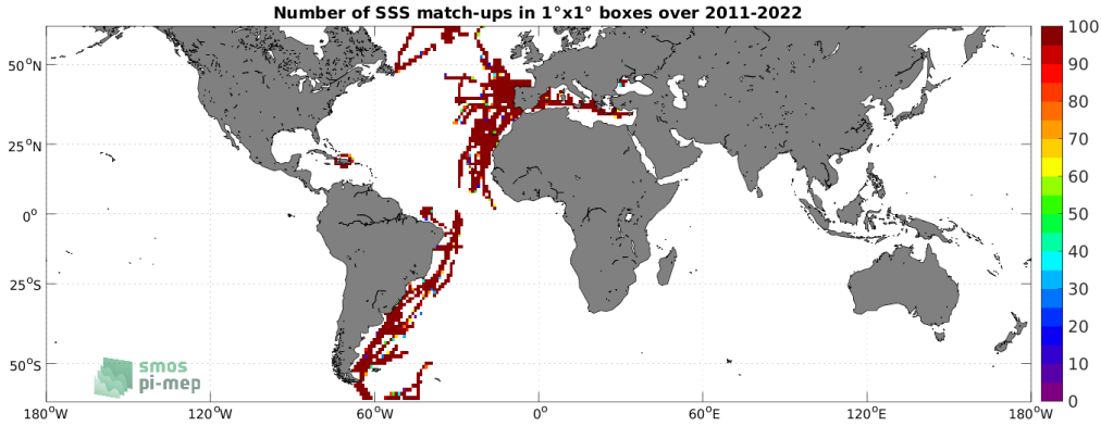
Figure 4: Number of SSS match-ups between TSG (CSIC-UTM) SSS and the SMAP SSS L4 OI v2 - 7 Days (ESR) SSS product for the SMOS coastal zone (<800km) 60N-60S Pi-MEP region over 1^\circ \times 1^\circ boxes and for the full satellite product period.
