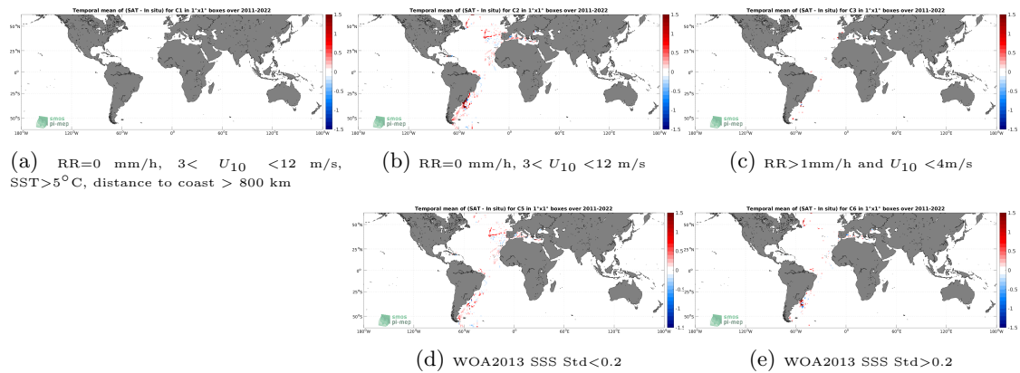
Figure 12: Temporal mean gridded over spatial boxes of size 1^\circ \times 1^\circ of \Delta SSS (SMAP SSS L4 OI v2 - 7 Days (ESR) - TSG (CSIC-UTM)) for 5 different subdatasets corresponding to:RR=0 mm/h, 3 < U_{10} < 12 m/s, SST >5^\circ\text{C} , distance to coast > 800 km (a), RR=0 mm/h, 3 < U_{10} < 12 m/s (b), RR >1 mm/h and U_{10} < 4 m/s (c), WOA2013 SSS Std <0.2 (d), WOA2013 SSS Std >0.2 (e).
