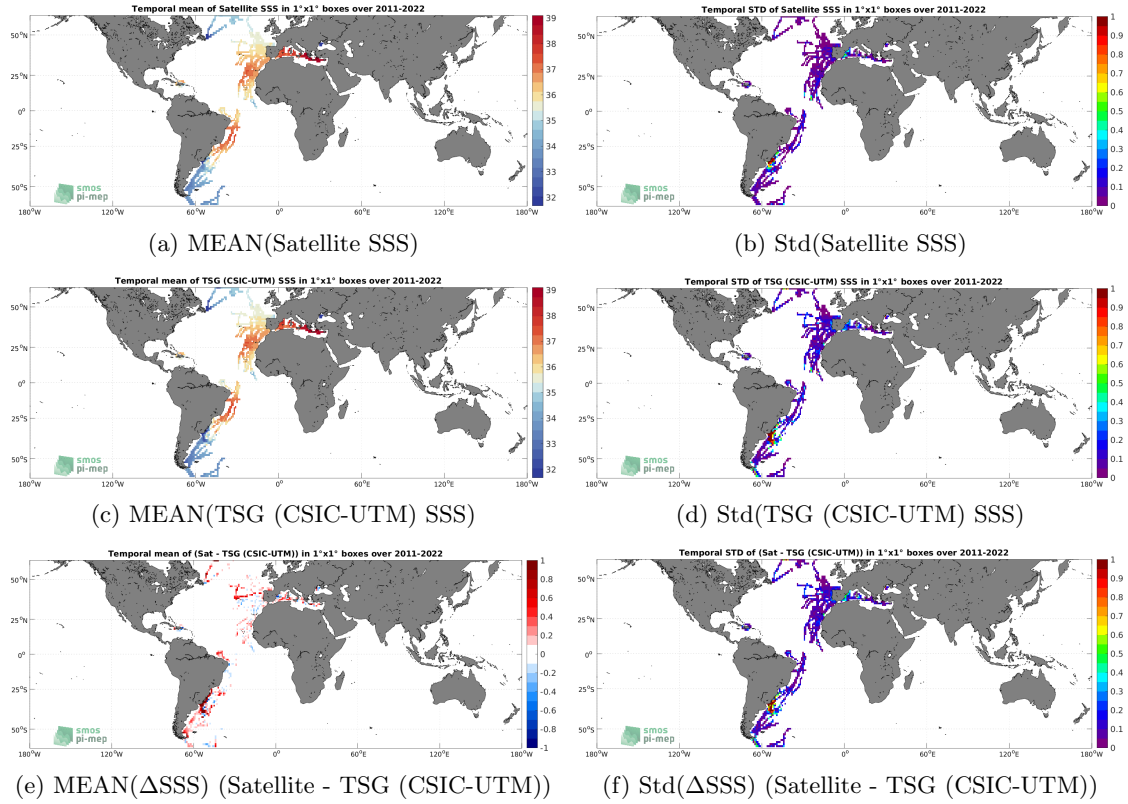
Figure 6: Temporal mean (left) and Std (right) of SSS from SMAP SSS L4 OI v2 - 7 Days (ESR) (top), TSG (CSIC-UTM) (middle), and of \Delta SSS (Satellite - TSG (CSIC-UTM)). Only match-up pairs are used to generate these maps.
