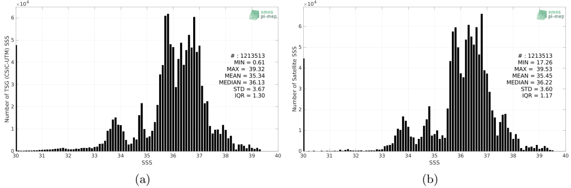
Figure 2: Histograms of SSS from TSG (CSIC-UTM) (a) and SMAP SSS L4 OI v2 - 7 Days (ESR) (b) considering all match-up pairs per bins of 0.1 over the SMOS coastal zone (<800km) 60N-60S Pi-MEP region and for the full satellite product period.
