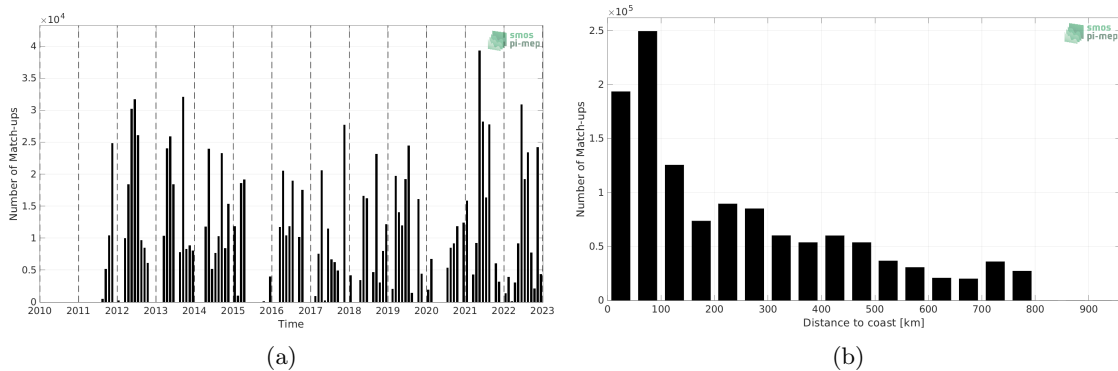
Figure 1: Number of match-ups between TSG (CSIC-UTM) and SMAP SSS L4 OI v2 - 7 Days (ESR) SSS as a function of time (a) and as function of the distance to coast (b) over the SMOS coastal zone (<800km) 60N-60S Pi-MEP region and for the full satellite product period.
