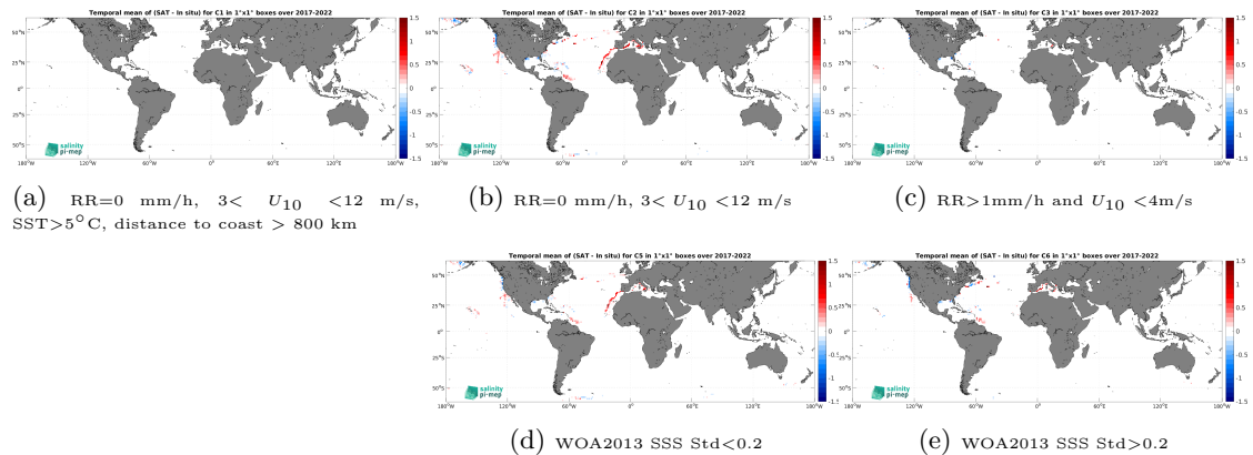
Figure 12: Temporal mean gridded over spatial boxes of size 1^\circ \times 1^\circ of \Delta SSS (SMAP SSS L4 OI v2 - 7 Days (ESR) - Saildrone) for 5 different subdatasets corresponding to:RR=0 mm/h, 3 < U_{10} < 12 m/s, SST >5^\circ\text{C} , distance to coast > 800 km (a), RR=0 mm/h, 3 < U_{10} < 12 m/s (b), RR >1 mm/h and U_{10} < 4 m/s (c), WOA2013 SSS Std <0.2 (d), WOA2013 SSS Std >0.2 (e).
