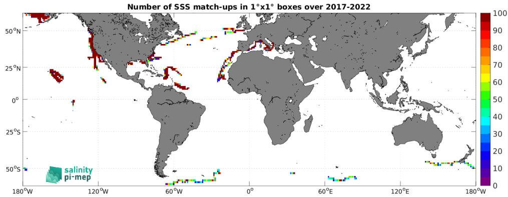
Figure 4: Number of SSS match-ups between Saildrone SSS and the SMAP SSS L4 OI v2 - 7 Days (ESR) SSS product for the SMOS coastal zone (<800km) 60N-60S Pi-MEP region over 1^\circ \times 1^\circ boxes and for the full satellite product period.
