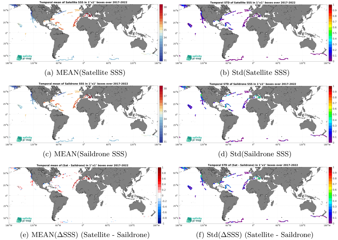
Figure 6: Temporal mean (left) and Std (right) of SSS from SMAP SSS L4 OI v2 - 7 Days (ESR) (top), Saildrone (middle), and of \Delta SSS (Satellite - Saildrone). Only match-up pairs are used to generate these maps.
