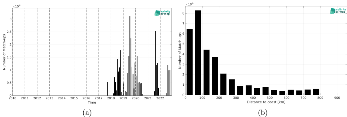
Figure 1: Number of match-ups between Saildrone and SMAP SSS L4 OI v2 - 7 Days (ESR) SSS as a function of time (a) and as function of the distance to coast (b) over the SMOS coastal zone ( < 800\text{km} ) 60\text{N}-60\text{S} Pi-MEP region and for the full satellite product period.
