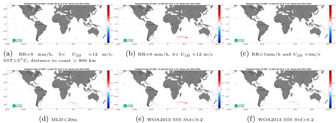
Figure 12: Temporal mean gridded over spatial boxes of size 1^\circ \times 1^\circ of \Delta SSS (SMAP SSS L4 OI v2 - 7 Days (ESR) - Marine mammals) for 6 different subdatasets corresponding to:RR=0 mm/h, 3 < U_{10} < 12 m/s, SST >5^\circ C, distance to coast > 800 km (a), RR=0 mm/h, 3 < U_{10} < 12 m/s (b), RR >1 mm/h and U_{10} < 4 m/s (c),MLD <20 m (d),WOA2013 SSS Std <0.2 (e),WOA2013 SSS Std >0.2 (f).
