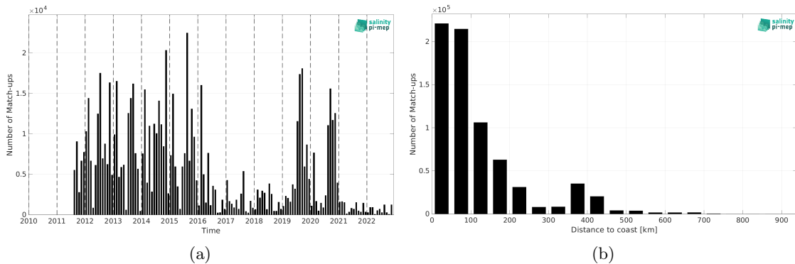
Figure 1: Number of match-ups between ICES and SMAP SSS L4 OI v2 - 7 Days (ESR) SSS as a function of time (a) and as function of the distance to coast (b) over the SMOS coastal zone ( < 800\text{km} ) 60N-60S Pi-MEP region and for the full satellite product period.
