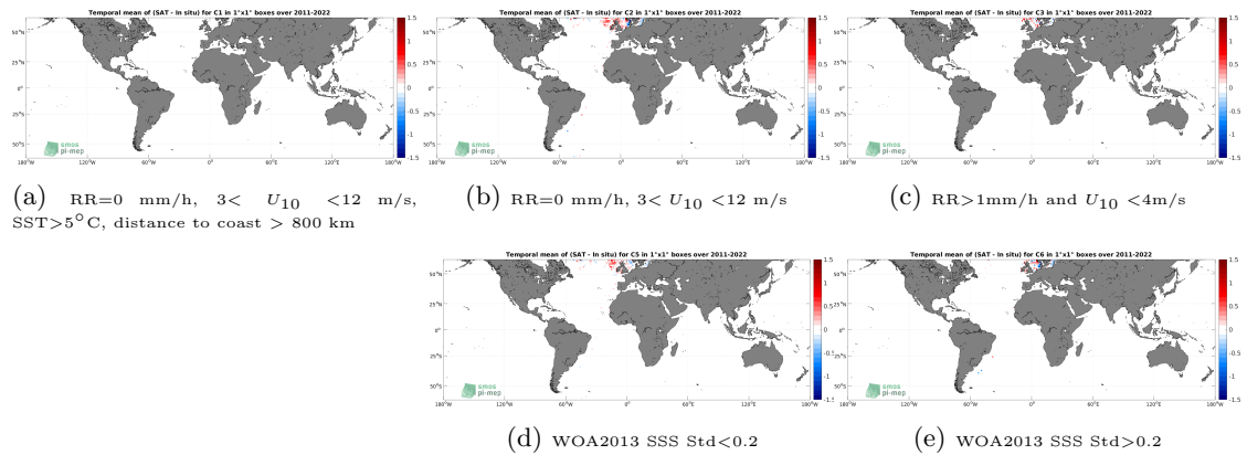
Figure 12: Temporal mean gridded over spatial boxes of size 1^\circ \times 1^\circ of \Delta SSS (SMAP SSS L4 OI v2 - 7 Days (ESR) - ICES) for 5 different subdatasets corresponding to:RR=0 mm/h, 3 < U_{10} < 12 m/s, SST >5^\circ\text{C} , distance to coast > 800 km (a), RR=0 mm/h, 3 < U_{10} < 12 m/s (b), RR >1 mm/h and U_{10} < 4 m/s (c), WOA2013 SSS Std <0.2 (d), WOA2013 SSS Std >0.2 (e).
