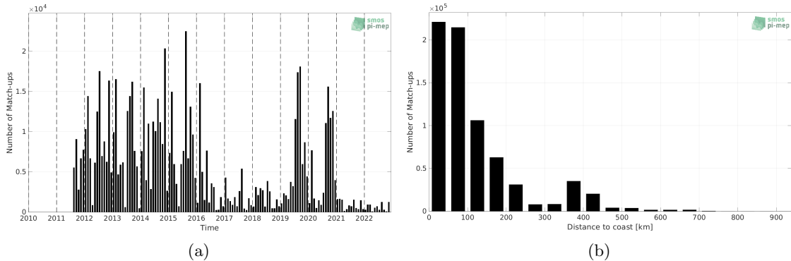
Figure 1: Number of match-ups between ICES and SMAP SSS L4 OI v2 - 7 Days (ESR) SSS as a function of time (a) and as function of the distance to coast (b) over the SMOS coastal zone (<800km) 60N-60S Pi-MEP region and for the full satellite product period.
