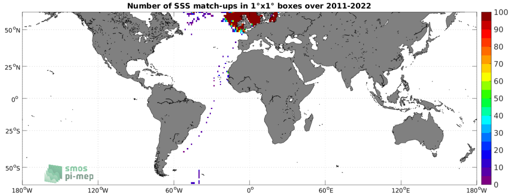
Figure 4: Number of SSS match-ups between ICES SSS and the SMAP SSS L4 OI v2 - 7 Days (ESR) SSS product for the SMOS coastal zone (<800km) 60N-60S Pi-MEP region over 1^\circ \times 1^\circ boxes and for the full satellite product period.
