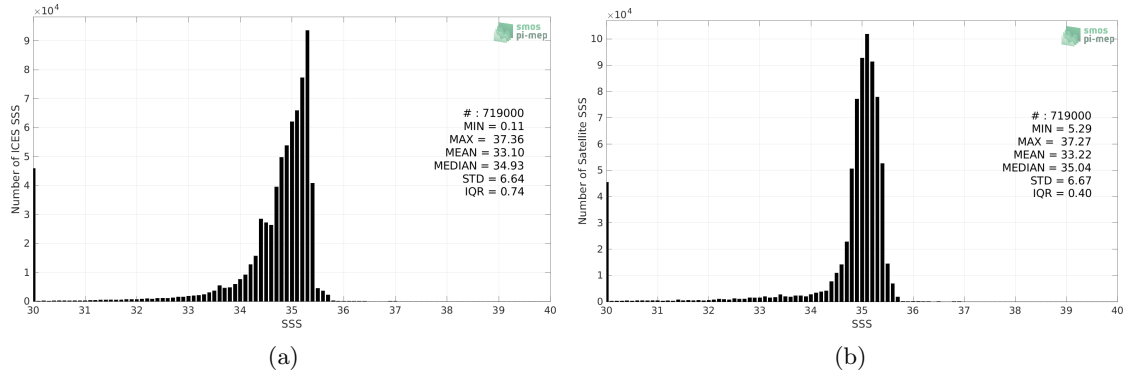
Figure 2: Histograms of SSS from ICES (a) and SMAP SSS L4 OI v2 - 7 Days (ESR) (b) considering all match-up pairs per bins of 0.1 over the SMOS coastal zone (<800km) 60N-60S Pi-MEP region and for the full satellite product period.
