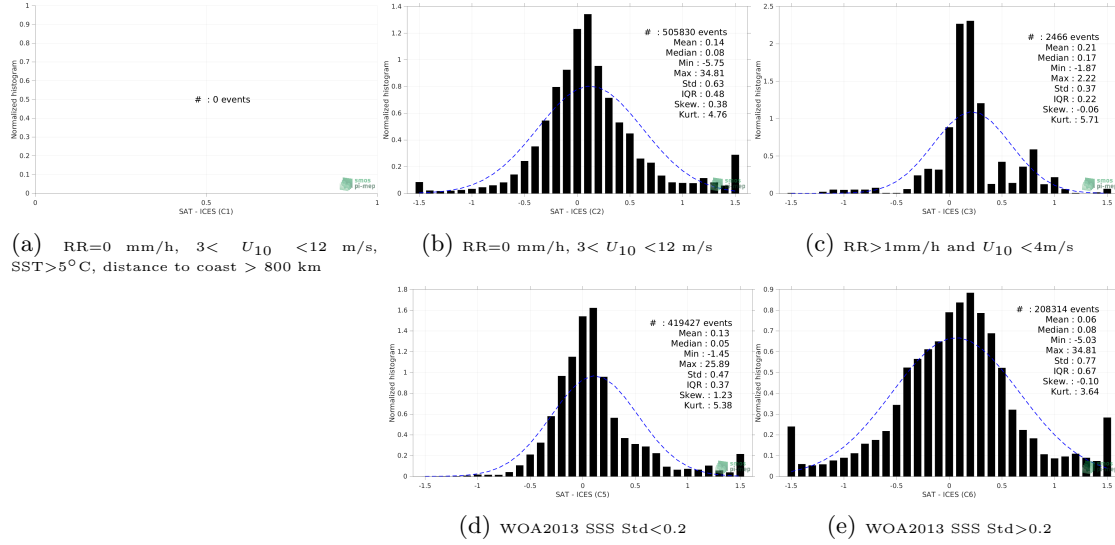
Figure 13: Normalized histogram of \Delta SSS (SMAP SSS L4 OI v2 - 7 Days (ESR) - ICES) for 5 different subdatasets corresponding to: RR=0 mm/h, 3 < U_{10} < 12 m/s, SST>5°C, distance to coast > 800 km (a), RR=0 mm/h, 3 < U_{10} < 12 m/s (b), RR>1mm/h and U_{10} < 4 m/s (c), WOA2013 SSS Std<0.2 (d), WOA2013 SSS Std>0.2 (e).
