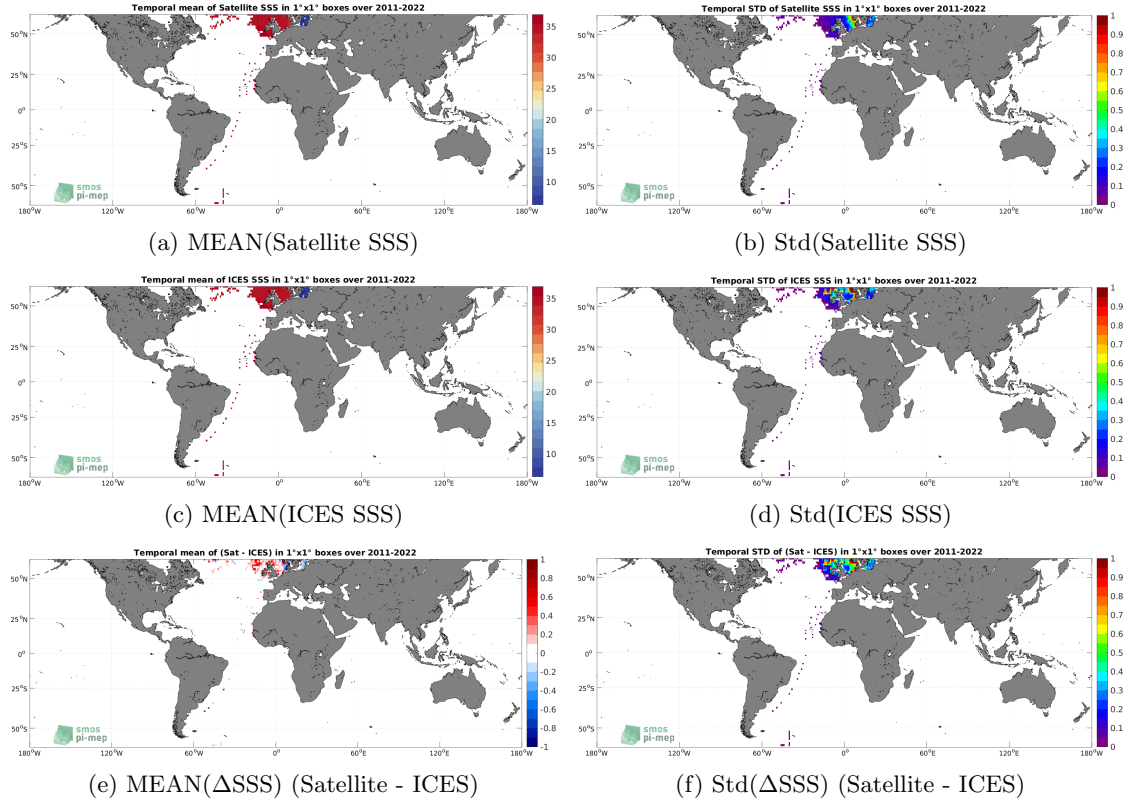
Figure 6: Temporal mean (left) and Std (right) of SSS from SMAP SSS L4 OI v2 - 7 Days (ESR) (top), ICES (middle), and of \Delta SSS (Satellite - ICES). Only match-up pairs are used to generate these maps.
