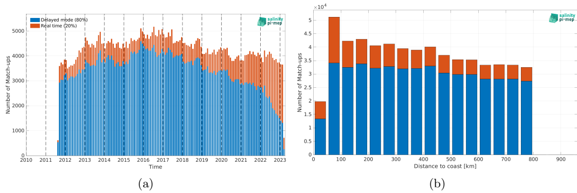
Figure 1: Number of match-ups between Argo and SMAP SSS L4 OI v2 - 7 Days (ESR) SSS as a function of time (a) and as function of the distance to coast (b) over the SMOS coastal zone (<800km) 60N-60S Pi-MEP region and for the full satellite product period.
