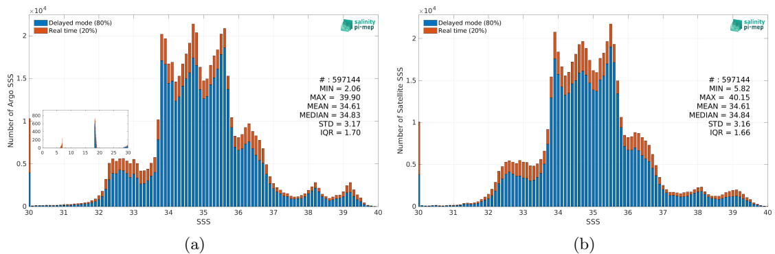
Figure 2: Histograms of SSS from Argo (a) and SMAP SSS L4 OI v2 - 7 Days (ESR) (b) considering all match-up pairs per bins of 0.1 over the SMOS coastal zone (<800km) 60N-60S Pi-MEP region and for the full satellite product period.
