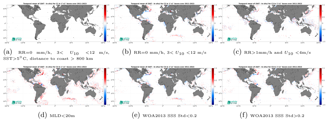
Figure 12: Temporal mean gridded over spatial boxes of size 1^\circ \times 1^\circ of \Delta SSS (SMAP SSS L4 OI v2 - 7 Days (ESR) - Argo) for 6 different subdatasets corresponding to:RR=0 mm/h, 3 < U_{10} < 12 m/s, SST >5^\circ C, distance to coast > 800 km (a), RR=0 mm/h, 3 < U_{10} < 12 m/s (b), RR >1 mm/h and U_{10} < 4 m/s (c),MLD <20 m (d),WOA2013 SSS Std <0.2 (e),WOA2013 SSS Std >0.2 (f).
