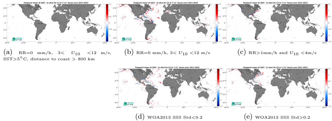
Figure 12: Temporal mean gridded over spatial boxes of size 1^\circ \times 1^\circ of \Delta\text{SSS} (SMAP SSS L4 OI v2 - Monthly (IPRC) - TSG (SAMOS)) for 5 different subdatasets corresponding to:RR=0 mm/h, 3 < U_{10} < 12 m/s, SST >5^\circ\text{C} , distance to coast > 800 km (a), RR=0 mm/h, 3 < U_{10} < 12 m/s (b), RR >1 mm/h and U_{10} < 4 m/s (c), WOA2013 SSS Std <0.2 (d), WOA2013 SSS Std >0.2 (e).
