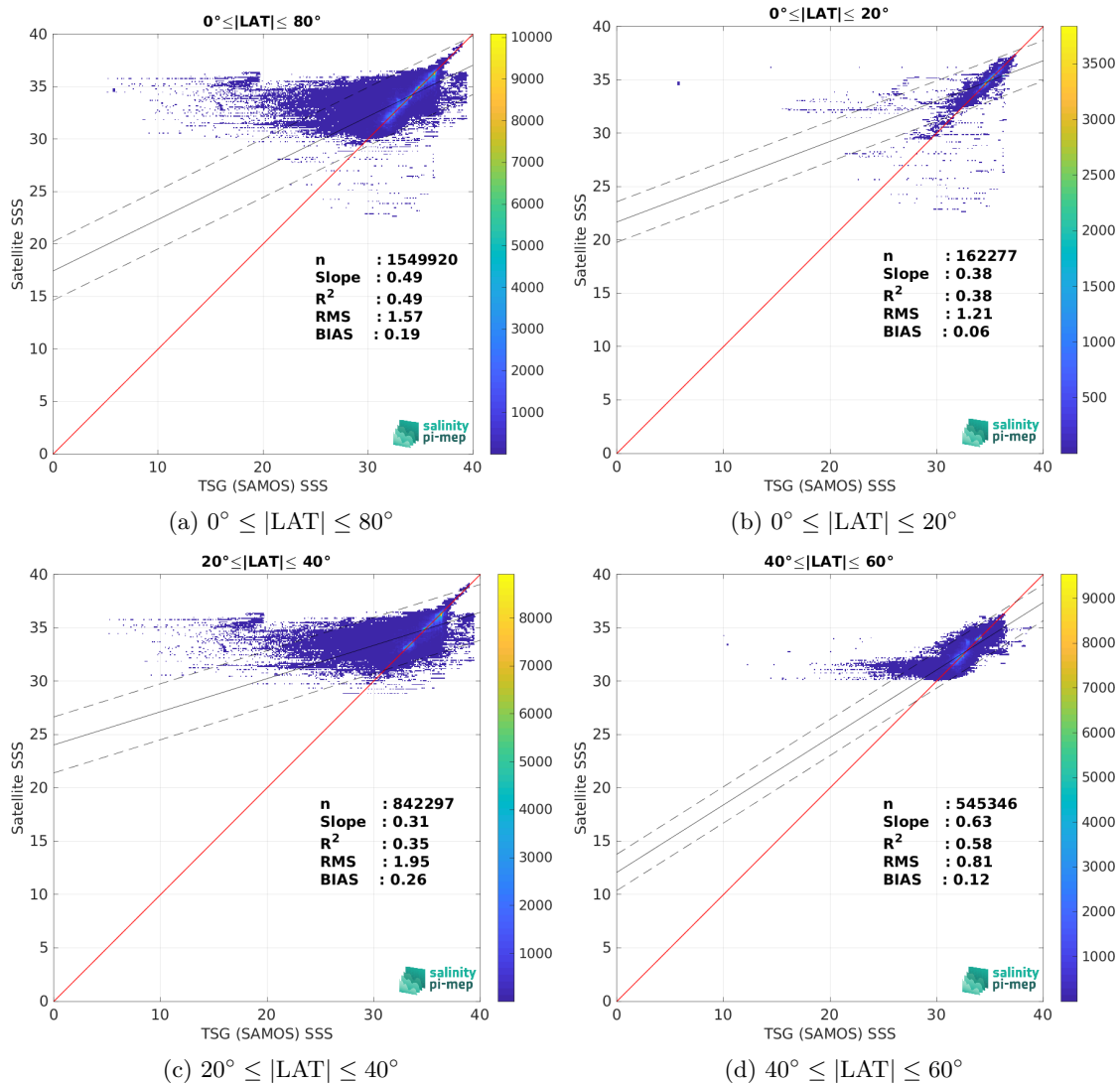
Figure 9: Contour maps of the concentration of SMAP SSS L4 OI v2 - Monthly (IPRC) SSS (y-axis) versus TSG (SAMOS) SSS (x-axis) at match-up pairs for different latitude bands. For each plot, the red line shows x=y . The black thin and dashed lines indicate a linear fit through the data cloud and the \pm 95\% confidence levels, respectively. The number match-up pairs n , the slope and R^2 coefficient of the linear fit, the root mean square (RMS) and the mean bias between satellite and in situ data are indicated for each latitude band in each plot.
