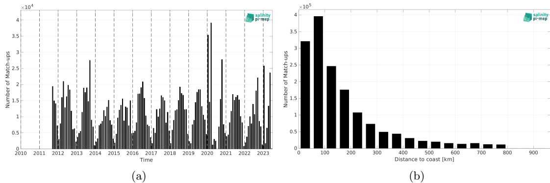
Figure 1: Number of match-ups between TSG (SAMOS) and SMAP SSS L4 OI v2 - Monthly (IPRC) SSS as a function of time (a) and as function of the distance to coast (b) over the SMOS coastal zone (<800km) 60N-60S Pi-MEP region and for the full satellite product period.
