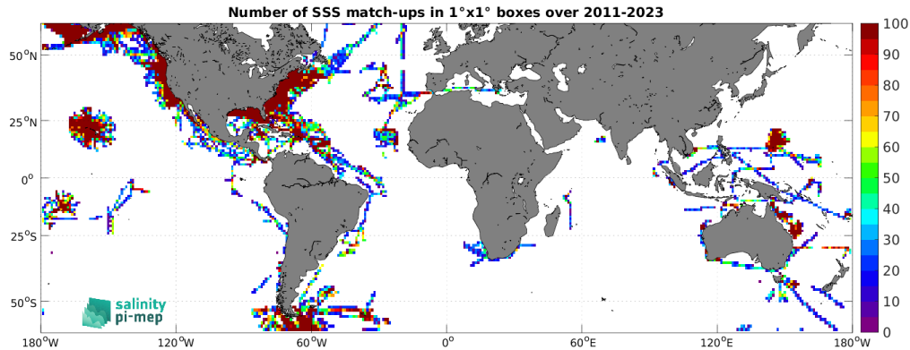
Figure 4: Number of SSS match-ups between TSG (SAMOS) SSS and the SMAP SSS L4 OI v2 - Monthly (IPRC) SSS product for the SMOS coastal zone (<800km) 60N-60S Pi-MEP region over 1^\circ \times 1^\circ boxes and for the full satellite product period.
