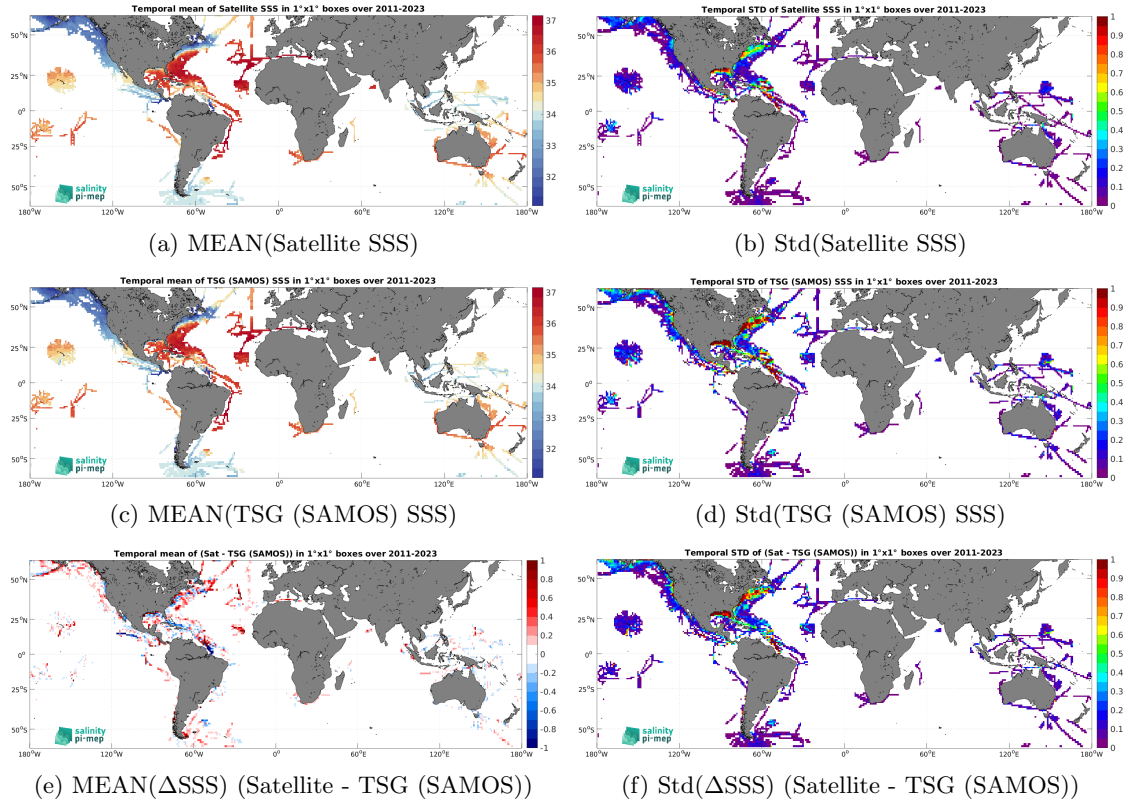
Figure 6: Temporal mean (left) and Std (right) of SSS from SMAP SSS L4 OI v2 - Monthly (IPRC) (top), TSG (SAMOS) (middle), and of \Delta SSS (Satellite - TSG (SAMOS)). Only match-up pairs are used to generate these maps.
