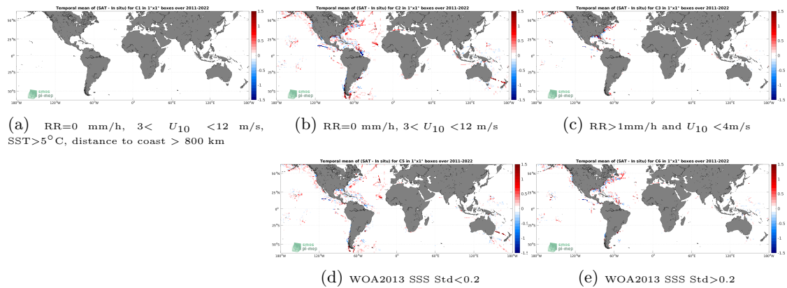
Figure 12: Temporal mean gridded over spatial boxes of size 1^\circ \times 1^\circ of \Delta SSS (SMAP SSS L4 OI v2 - Monthly (IPRC) - TSG (SAMOS)) for 5 different subdatasets corresponding to:RR=0 mm/h, 3 < U_{10} < 12 m/s, SST >5^\circ\text{C} , distance to coast > 800 km (a), RR=0 mm/h, 3 < U_{10} < 12 m/s (b), RR >1 mm/h and U_{10} < 4 m/s (c), WOA2013 SSS Std <0.2 (d), WOA2013 SSS Std >0.2 (e).
