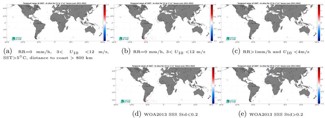
Figure 12: Temporal mean gridded over spatial boxes of size 1^\circ \times 1^\circ of \Delta\text{SSS} (SMAP SSS L4 OI v2 - Monthly (IPRC) - TSG (Polarstern)) for 5 different subdatasets corresponding to:RR=0 mm/h, 3 < U_{10} < 12 m/s, SST >5^\circ\text{C} , distance to coast > 800 km (a), RR=0 mm/h, 3 < U_{10} < 12 m/s (b), RR >1 mm/h and U_{10} < 4 m/s (c), WOA2013 SSS Std <0.2 (d), WOA2013 SSS Std >0.2 (e).
