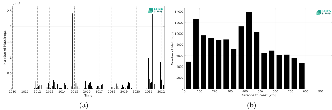
Figure 1: Number of match-ups between TSG (Polarstern) and SMAP SSS L4 OI v2 - Monthly (IPRC) SSS as a function of time (a) and as function of the distance to coast (b) over the SMOS coastal zone (<800km) 60N-60S Pi-MEP region and for the full satellite product period.
