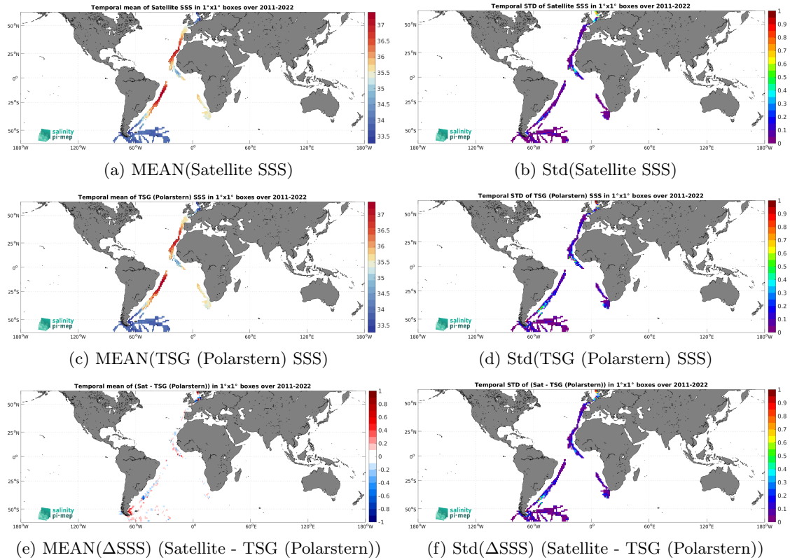
Figure 6: Temporal mean (left) and Std (right) of SSS from SMAP SSS L4 OI v2 - Monthly (IPRC) (top), TSG (Polarstern) (middle), and of \Delta SSS (Satellite - TSG (Polarstern)). Only match-up pairs are used to generate these maps.
