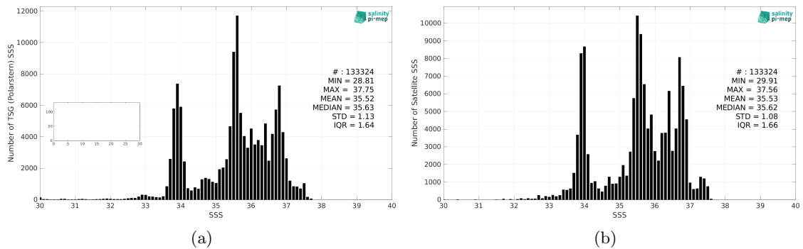
Figure 2: Histograms of SSS from TSG (Polarstern) (a) and SMAP SSS L4 OI v2 - Monthly (IPRC) (b) considering all match-up pairs per bins of 0.1 over the SMOS coastal zone (<800km) 60N-60S Pi-MEP region and for the full satellite product period.
