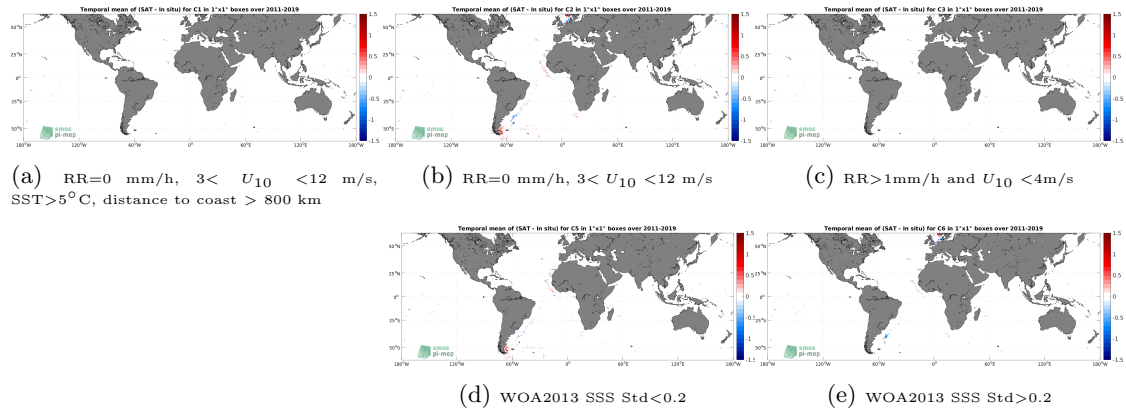
Figure 12: Temporal mean gridded over spatial boxes of size 1^\circ \times 1^\circ of \Delta SSS (SMAP SSS L4 OI v2 - Monthly (IPRC) - TSG (Polarstern)) for 5 different subdatasets corresponding to:RR=0 mm/h, 3 < U_{10} < 12 m/s, SST >5^\circ\text{C} , distance to coast > 800 km (a), RR=0 mm/h, 3 < U_{10} < 12 m/s (b), RR >1 mm/h and U_{10} < 4 m/s (c), WOA2013 SSS Std <0.2 (d), WOA2013 SSS Std >0.2 (e).
