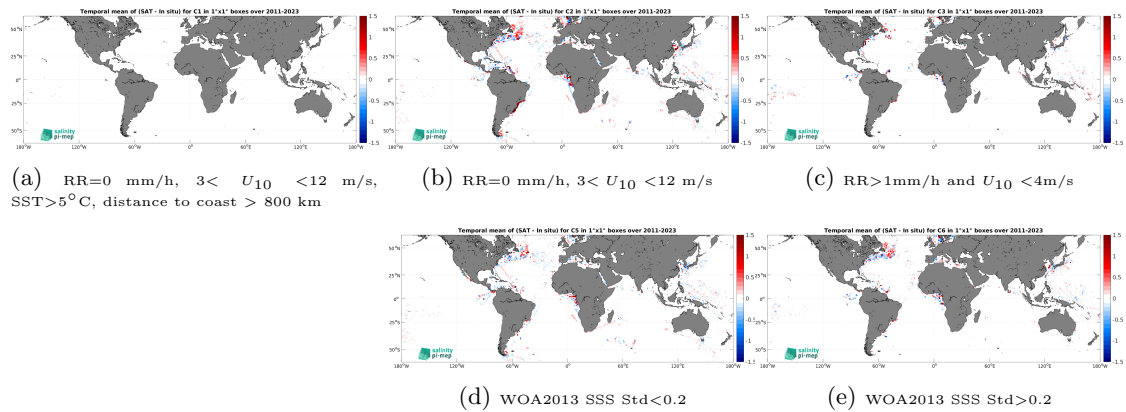
Figure 12: Temporal mean gridded over spatial boxes of size 1^\circ \times 1^\circ of \Delta\text{SSS} (SMAP SSS L4 OI v2 - Monthly (IPRC) - TSG (LEGOS-DM)) for 5 different subdatasets corresponding to:RR=0 mm/h, 3 < U_{10} < 12 m/s, SST >5^\circ\text{C} , distance to coast > 800 km (a), RR=0 mm/h, 3 < U_{10} < 12 m/s (b), RR >1 mm/h and U_{10} < 4 m/s (c), WOA2013 SSS Std <0.2 (d), WOA2013 SSS Std >0.2 (e).
