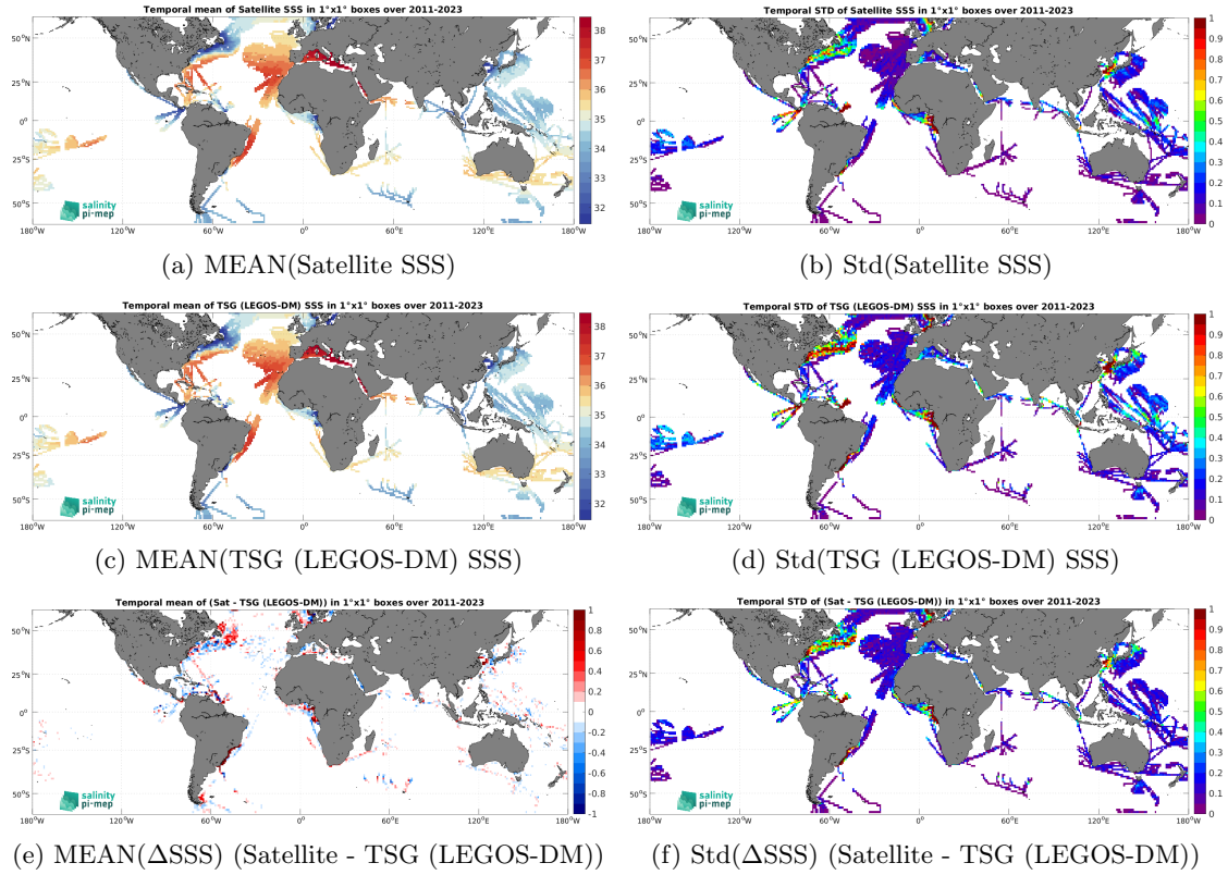
Figure 6: Temporal mean (left) and Std (right) of SSS from SMAP SSS L4 OI v2 - Monthly (IPRC) (top), TSG (LEGOS-DM) (middle), and of \Delta SSS (Satellite - TSG (LEGOS-DM)). Only match-up pairs are used to generate these maps.
