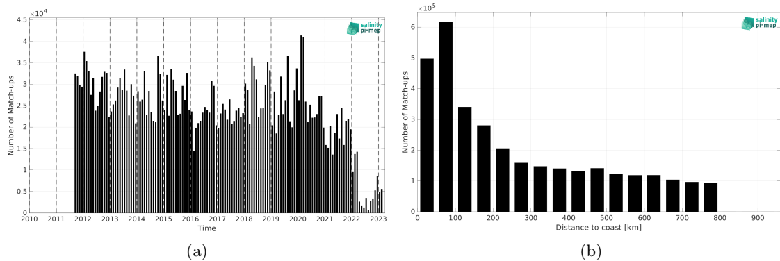
Figure 1: Number of match-ups between TSG (LEGOS-DM) and SMAP SSS L4 OI v2 - Monthly (IPRC) SSS as a function of time (a) and as function of the distance to coast (b) over the SMOS coastal zone (<800km) 60N-60S Pi-MEP region and for the full satellite product period.
