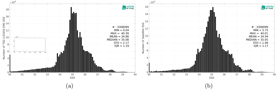
Figure 2: Histograms of SSS from TSG (LEGOS-DM) (a) and SMAP SSS L4 OI v2 - Monthly (IPRC) (b) considering all match-up pairs per bins of 0.1 over the SMOS coastal zone (<800km) 60N-60S Pi-MEP region and for the full satellite product period.
