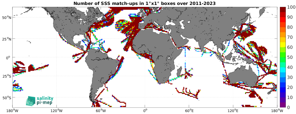
Figure 4: Number of SSS match-ups between TSG (LEGOS-DM) SSS and the SMAP SSS L4 OI v2 - Monthly (IPRC) SSS product for the SMOS coastal zone (<800km) 60N-60S Pi-MEP region over 1^{\circ} \times 1^{\circ} boxes and for the full satellite product period.
