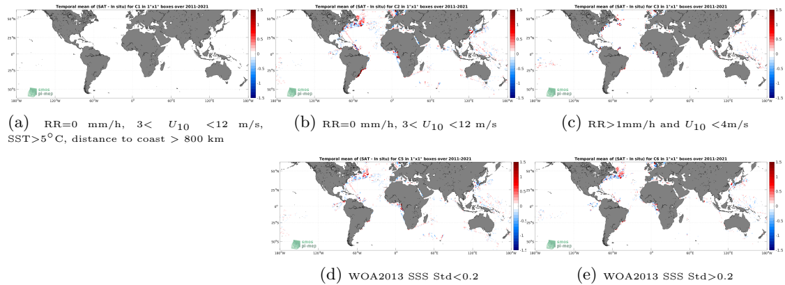
Figure 12: Temporal mean gridded over spatial boxes of size 1^\circ \times 1^\circ of \Delta SSS (SMAP SSS L4 OI v2 - Monthly (IPRC) - TSG (LEGOS-DM)) for 5 different subdatasets corresponding to:RR=0 mm/h, 3 < U_{10} < 12 m/s, SST >5^\circ\text{C} , distance to coast > 800 km (a), RR=0 mm/h, 3 < U_{10} < 12 m/s (b), RR >1 mm/h and U_{10} < 4 m/s (c), WOA2013 SSS Std <0.2 (d), WOA2013 SSS Std >0.2 (e).
