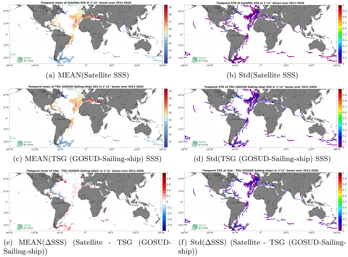
Figure 6: Temporal mean (left) and Std (right) of SSS from SMAP SSS L4 OI v2 - Monthly (IPRC) (top), TSG (GOSUD-Sailing-ship) (middle), and of \Delta SSS (Satellite - TSG (GOSUD-Sailing-ship)). Only match-up pairs are used to generate these maps.
