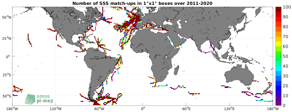
Figure 4: Number of SSS match-ups between TSG (GOSUD-Sailing-ship) SSS and the SMAP SSS L4 OI v2 - Monthly (IPRC) SSS product for the SMOS coastal zone (<800km) 60N-60S Pi-MEP region over 1^{\circ} \times 1^{\circ} boxes and for the full satellite product period.
