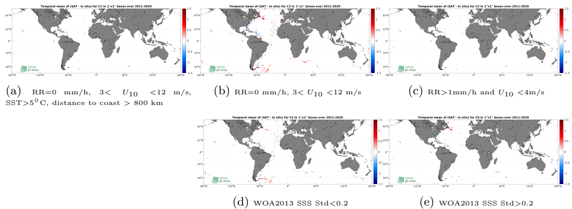
Figure 12: Temporal mean gridded over spatial boxes of size 1^\circ \times 1^\circ of \Delta\text{SSS} (SMAP SSS L4 OI v2 - Monthly (IPRC) - TSG (GOSUD-Sailing-ship)) for 5 different subdatasets corresponding to:RR=0 mm/h, 3 < U_{10} < 12 m/s, SST>5°C, distance to coast > 800 km (a), RR=0 mm/h, 3 < U_{10} < 12 m/s (b), RR>1mm/h and U_{10} < 4 m/s (c), WOA2013 SSS Std<0.2 (d), WOA2013 SSS Std>0.2 (e).
