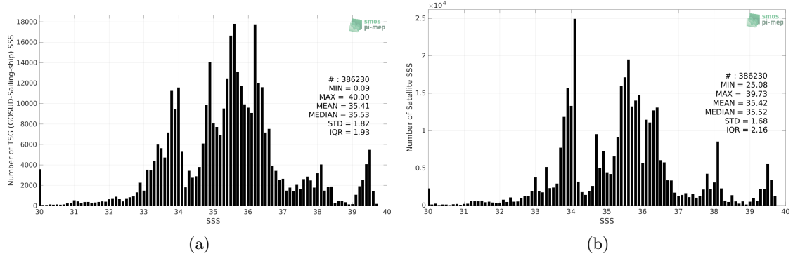
Figure 2: Histograms of SSS from TSG (GOSUD-Sailing-ship) (a) and SMAP SSS L4 OI v2 - Monthly (IPRC) (b) considering all match-up pairs per bins of 0.1 over the SMOS coastal zone (<800km) 60N-60S Pi-MEP region and for the full satellite product period.
