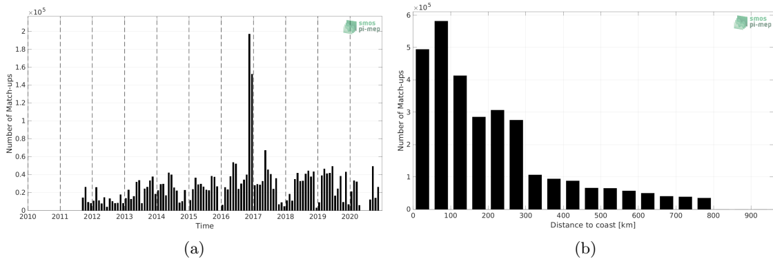
Figure 1: Number of match-ups between TSG (GOSUD-Research-vessel) and SMAP SSS L4 OI v2 - Monthly (IPRC) SSS as a function of time (a) and as function of the distance to coast (b) over the SMOS coastal zone (<800km) 60N-60S Pi-MEP region and for the full satellite product period.
