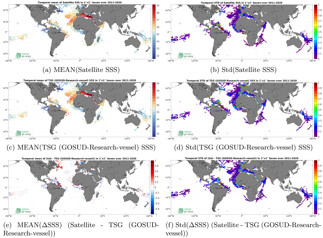
Figure 6: Temporal mean (left) and Std (right) of SSS from SMAP SSS L4 OI v2 - Monthly (IPRC) (top), TSG (GOSUD-Research-vessel) (middle), and of \Delta SSS (Satellite - TSG (GOSUD-Research-vessel)). Only match-up pairs are used to generate these maps.
