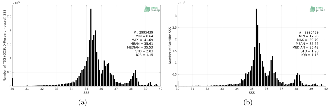
Figure 2: Histograms of SSS from TSG (GOSUD-Research-vessel) (a) and SMAP SSS L4 OI v2 - Monthly (IPRC) (b) considering all match-up pairs per bins of 0.1 over the SMOS coastal zone (<800km) 60N-60S Pi-MEP region and for the full satellite product period.
