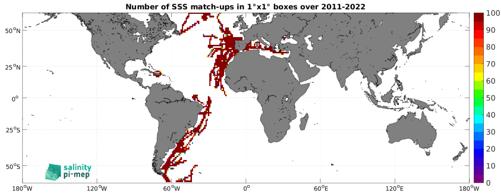
Figure 4: Number of SSS match-ups between TSG (CSIC-UTM) SSS and the SMAP SSS L4 OI v2 - Monthly (IPRC) SSS product for the SMOS coastal zone (<800km) 60N-60S Pi-MEP region over 1^{\circ} \times 1^{\circ} boxes and for the full satellite product period.
