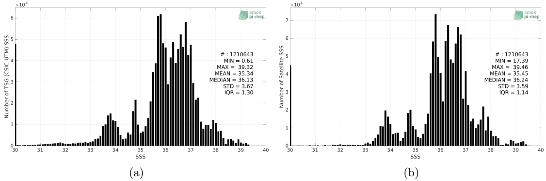
Figure 2: Histograms of SSS from TSG (CSIC-UTM) (a) and SMAP SSS L4 OI v2 - Monthly (IPRC) (b) considering all match-up pairs per bins of 0.1 over the SMOS coastal zone (<800km) 60N-60S Pi-MEP region and for the full satellite product period.
