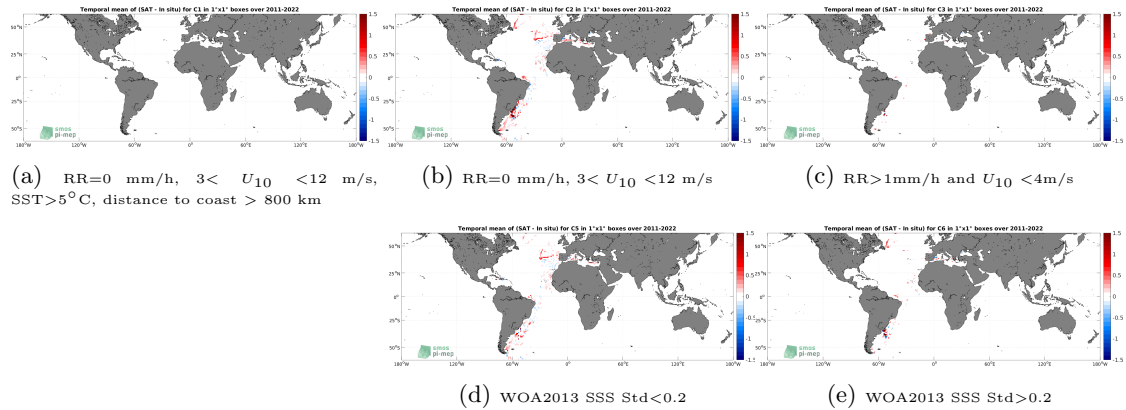
Figure 12: Temporal mean gridded over spatial boxes of size 1^\circ \times 1^\circ of \Delta SSS (SMAP SSS L4 OI v2 - Monthly (IPRC) - TSG (CSIC-UTM)) for 5 different subdatasets corresponding to:RR=0 mm/h, 3 < U_{10} < 12 m/s, SST >5^\circ\text{C} , distance to coast > 800 km (a), RR=0 mm/h, 3 < U_{10} < 12 m/s (b), RR >1 mm/h and U_{10} < 4 m/s (c), WOA2013 SSS Std <0.2 (d), WOA2013 SSS Std >0.2 (e).
