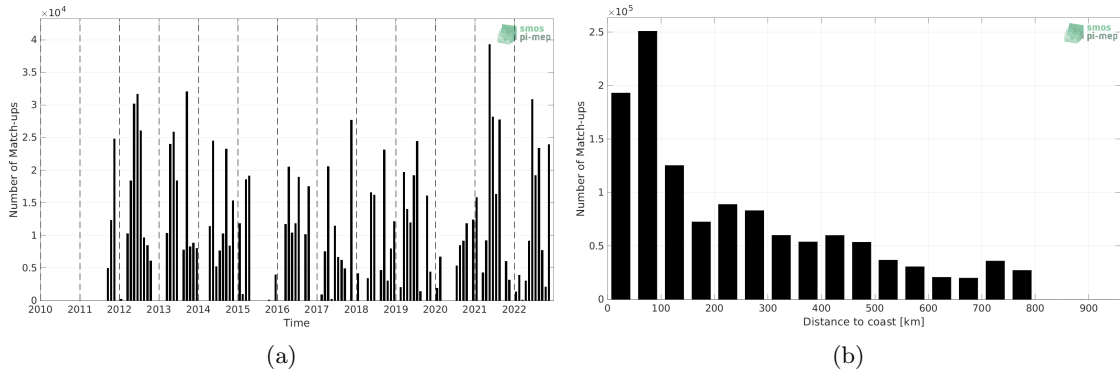
Figure 1: Number of match-ups between TSG (CSIC-UTM) and SMAP SSS L4 OI v2 - Monthly (IPRC) SSS as a function of time (a) and as function of the distance to coast (b) over the SMOS coastal zone (<800km) 60N-60S Pi-MEP region and for the full satellite product period.
