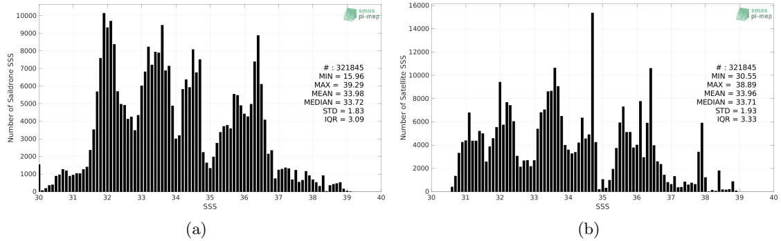
Figure 2: Histograms of SSS from Sairdrone (a) and SMAP SSS L4 OI v2 - Monthly (IPRC) (b) considering all match-up pairs per bins of 0.1 over the SMOS coastal zone (<800km) 60N-60S Pi-MEP region and for the full satellite product period.
