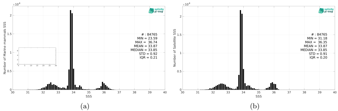
Figure 2: Histograms of SSS from Marine mammals (a) and SMAP SSS L4 OI v2 - Monthly (IPRC) (b) considering all match-up pairs per bins of 0.1 over the SMOS coastal zone (<800km) 60N-60S Pi-MEP region and for the full satellite product period.
