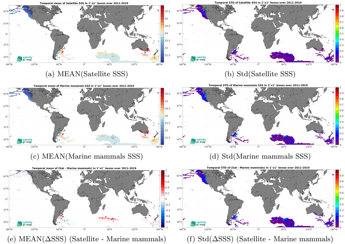
Figure 6: Temporal mean (left) and Std (right) of SSS from SMAP SSS L4 OI v2 - Monthly (IPRC) (top), Marine mammals (middle), and of \Delta SSS (Satellite - Marine mammals). Only match-up pairs are used to generate these maps.
