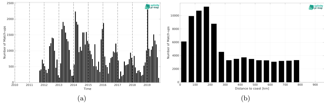
Figure 1: Number of match-ups between Marine mammals and SMAP SSS L4 OI v2 - Monthly (IPRC) SSS as a function of time (a) and as function of the distance to coast (b) over the SMOS coastal zone (<800km) 60N-60S Pi-MEP region and for the full satellite product period.
