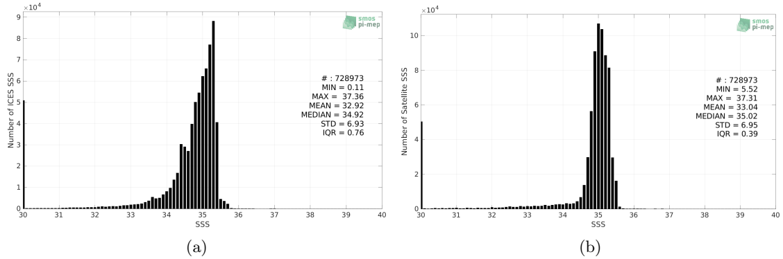
Figure 2: Histograms of SSS from ICES (a) and SMAP SSS L4 OI v2 - Monthly (IPRC) (b) considering all match-up pairs per bins of 0.1 over the SMOS coastal zone (<800km) 60N-60S Pi-MEP region and for the full satellite product period.
