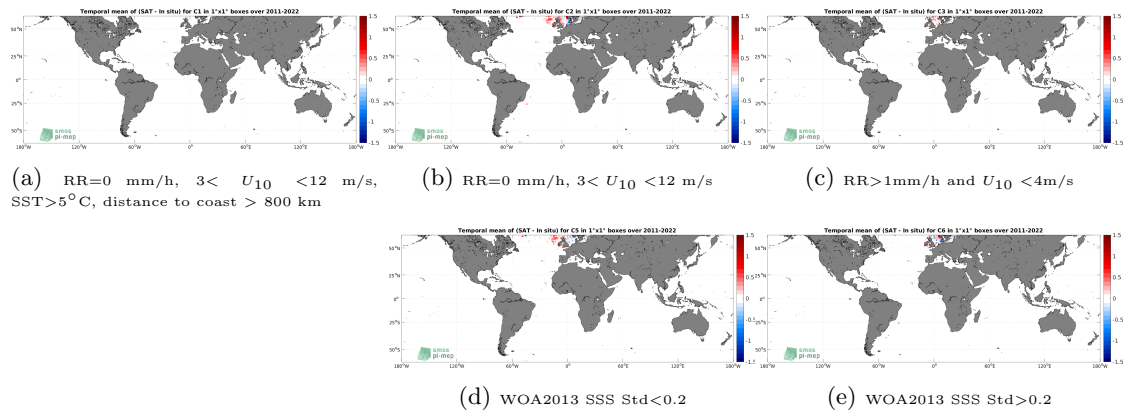
Figure 12: Temporal mean gridded over spatial boxes of size 1^\circ \times 1^\circ of \Delta SSS (SMAP SSS L4 OI v2 - Monthly (IPRC) - ICES) for 5 different subdatasets corresponding to:RR=0 mm/h, 3 < U_{10} < 12 m/s, SST >5^\circ\text{C} , distance to coast > 800 km (a), RR=0 mm/h, 3 < U_{10} < 12 m/s (b), RR >1 mm/h and U_{10} < 4 m/s (c), WOA2013 SSS Std <0.2 (d), WOA2013 SSS Std >0.2 (e).
