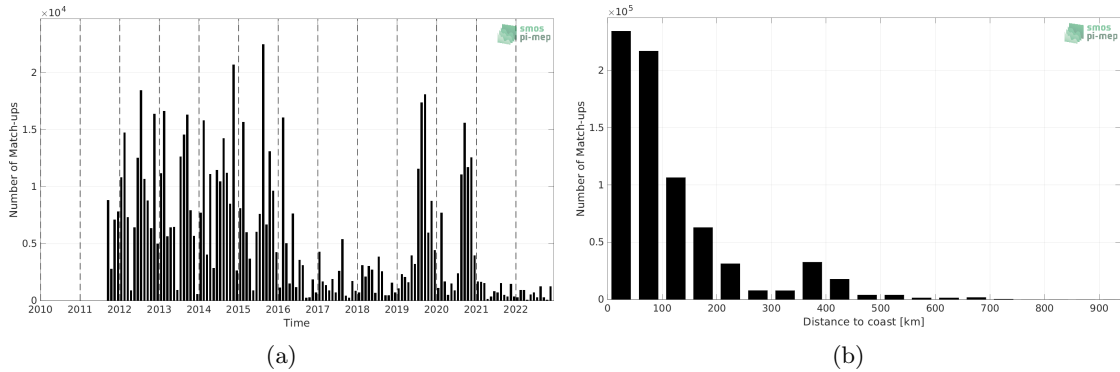
Figure 1: Number of match-ups between ICES and SMAP SSS L4 OI v2 - Monthly (IPRC) SSS as a function of time (a) and as function of the distance to coast (b) over the SMOS coastal zone (<800km) 60N-60S Pi-MEP region and for the full satellite product period.
