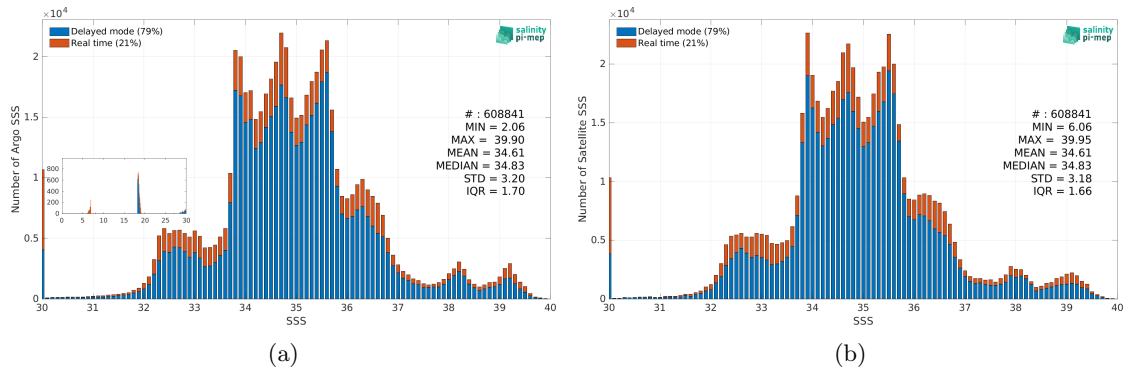
Figure 2: Histograms of SSS from Argo (a) and SMAP SSS L4 OI v2 - Monthly (IPRC) (b) considering all match-up pairs per bins of 0.1 over the SMOS coastal zone (<800km) 60N-60S Pi-MEP region and for the full satellite product period.
