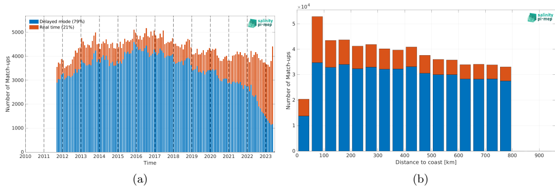
Figure 1: Number of match-ups between Argo and SMAP SSS L4 OI v2 - Monthly (IPRC) SSS as a function of time (a) and as function of the distance to coast (b) over the SMOS coastal zone (<800km) 60N-60S Pi-MEP region and for the full satellite product period.
