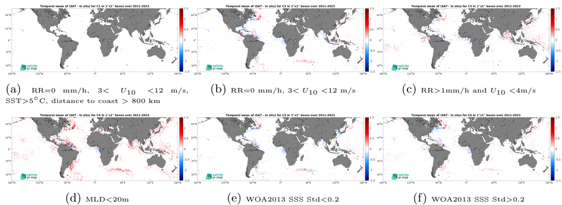
Figure 12: Temporal mean gridded over spatial boxes of size 1^\circ \times 1^\circ of \Delta SSS (SMAP SSS L4 OI v2 - Monthly (IPRC) - Argo) for 6 different subdatasets corresponding to:RR=0 mm/h, 3 < U_{10} < 12 m/s, SST >5^\circ C, distance to coast > 800 km (a), RR=0 mm/h, 3 < U_{10} < 12 m/s (b), RR >1 mm/h and U_{10} < 4 m/s (c),MLD <20 m (d),WOA2013 SSS Std <0.2 (e),WOA2013 SSS Std >0.2 (f).
