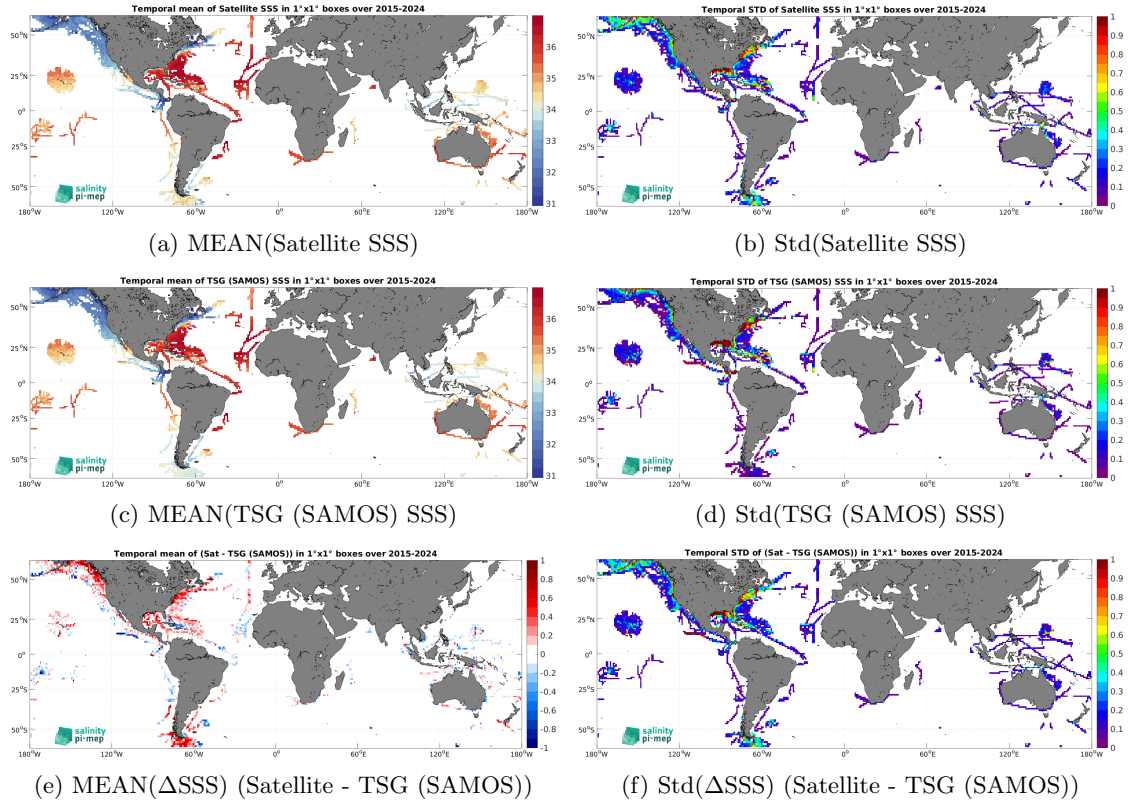
Figure 7: Temporal mean (left) and Std (right) of SSS from SMAP SSS L3 v6 - 8-Day running (RSS) (top), TSG (SAMOS) (middle), and of \Delta SSS (Satellite - TSG (SAMOS)). Only match-up pairs are used to generate these maps.
