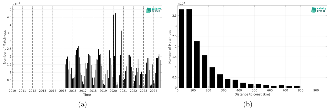
Figure 2: Number of match-ups between TSG (SAMOS) and SMAP SSS L3 v6 - 8-Day running (RSS) SSS as a function of time (a) and as function of the distance to coast (b) over the SMOS coastal zone (<800km) 60N-60S Pi-MEP region and for the full satellite product period.
