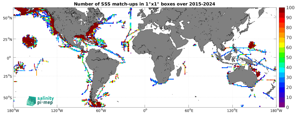
Figure 5: Number of SSS match-ups between TSG (SAMOS) SSS and the SMAP SSS L3 v6 - 8-Day running (RSS) SSS product for the SMOS coastal zone (<800km) 60N-60S Pi-MEP region over 1^\circ \times 1^\circ boxes and for the full satellite product period.
