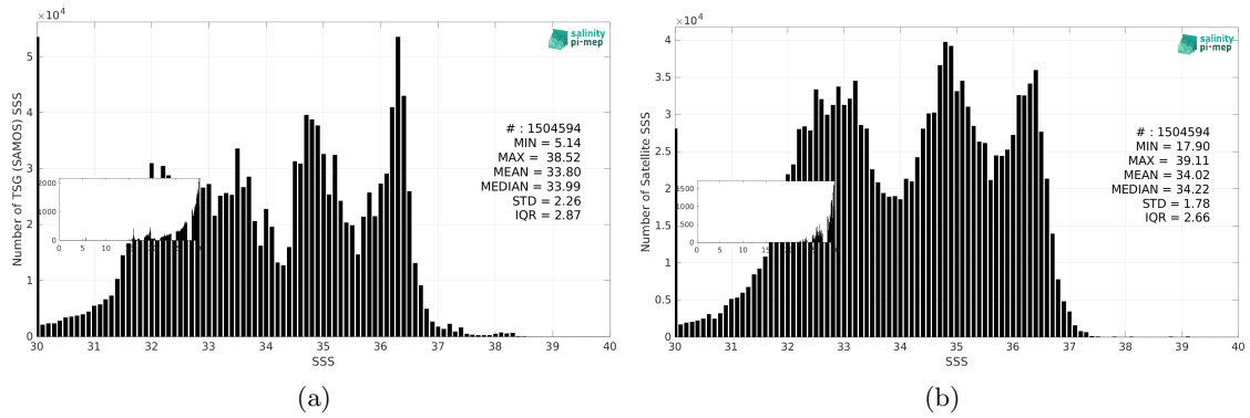
Figure 3: Histograms of SSS from TSG (SAMOS) (a) and SMAP SSS L3 v6 - 8-Day running (RSS) (b) considering all match-up pairs per bins of 0.1 over the SMOS coastal zone (<800km) 60N-60S Pi-MEP region and for the full satellite product period.
