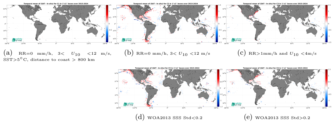
Figure 14: Temporal mean gridded over spatial boxes of size 1^\circ \times 1^\circ of \Delta SSS (SMAP SSS L3 v6 - 8-Day running (RSS) - TSG (SAMOS)) for 5 different subdatasets corresponding to:RR=0 mm/h, 3 < U_{10} < 12 m/s, SST >5^\circ\text{C} , distance to coast > 800 km (a), RR=0 mm/h, 3 < U_{10} < 12 m/s (b), RR >1 mm/h and U_{10} < 4 m/s (c), WOA2013 SSS Std <0.2 (d), WOA2013 SSS Std >0.2 (e).
