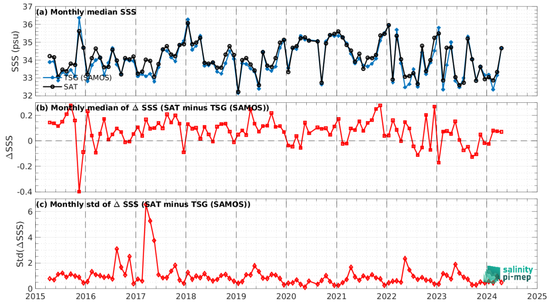
Figure 8: Time series of the monthly median SSS (top), median of \Delta SSS (Satellite - TSG (SAMOS)) and Std of \Delta SSS (Satellite - TSG (SAMOS)) over the SMOS coastal zone ( <800\text{km} ) 60N-60S Pi-MEP region considering all match-ups collected by the Pi-MEP.
